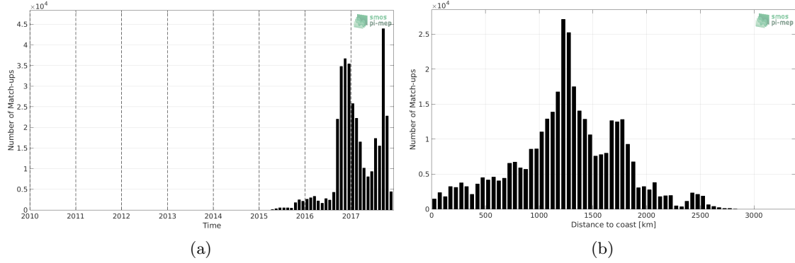
Figure 1: Number of match-ups between Surface drifters and SMAP-L3-RSS-V4-8DAY-RUNNING SSS as a function of time (a) and as function of the distance to coast (b) over the Tropical Pacific Ocean Pi-MEP region and for the full satellite product period.
