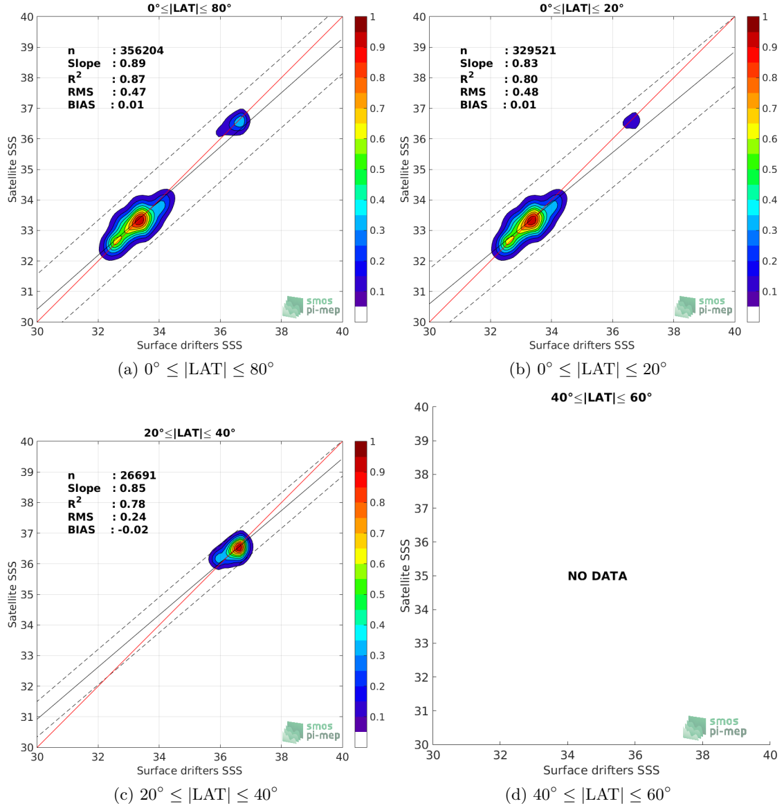
Figure 8: Contour maps of the concentration of SMAP-L3-RSS-V4-8DAY-RUNNING SSS (y-axis) versus Surface drifters SSS (x-axis) at match-up pairs for different latitude bands. For each plot, the red line shows x=y . The black thin and dashed lines indicate a linear fit through the data cloud and the \pm 95\% confidence levels, respectively. The number match-up pairs n , the slope and R^2 coefficient of the linear fit, the root mean square (RMS) and the mean bias between satellite and in situ data are indicated for each latitude band in each plots.
