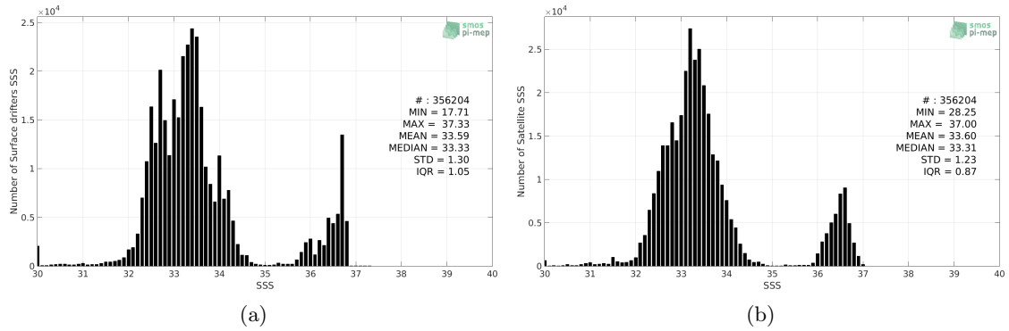
Figure 2: Histograms of SSS from Surface drifters (a) and SMAP-L3-RSS-V4-8DAY-RUNNING (b) considering all match-up pairs per bins of 0.1 over the Tropical Pacific Ocean Pi-MEP region and for the full satellite product period.
