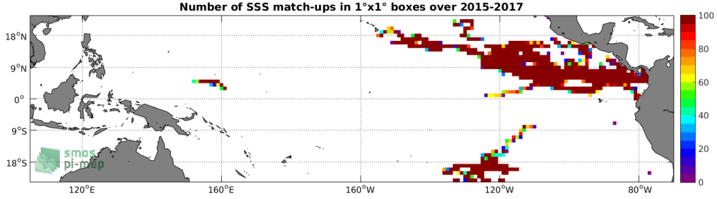
Figure 3: Number of SSS match-ups between Surface drifters SSS and the SMAP-L3-RSS-V4-8DAY-RUNNING SSS product for the Tropical Pacific Ocean Pi-MEP region over 1^\circ \times 1^\circ boxes and for the full satellite product period.
