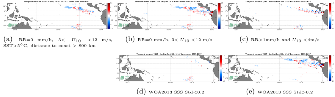
Figure 11: Temporal mean gridded over spatial boxes of size 1^\circ \times 1^\circ of \Delta SSS (SMAP-L3-RSS-V4-8DAY-RUNNING - Surface drifters) for 5 different subdatasets corresponding to: RR=0 mm/h, 3 < U_{10} < 12 m/s, SST >5^\circ\text{C} , distance to coast > 800 km (a), RR=0 mm/h, 3 < U_{10} < 12 m/s (b), RR >1 mm/h and U_{10} < 4 m/s (c), WOA2013 SSS Std <0.2 (d), WOA2013 SSS Std >0.2 (e).
