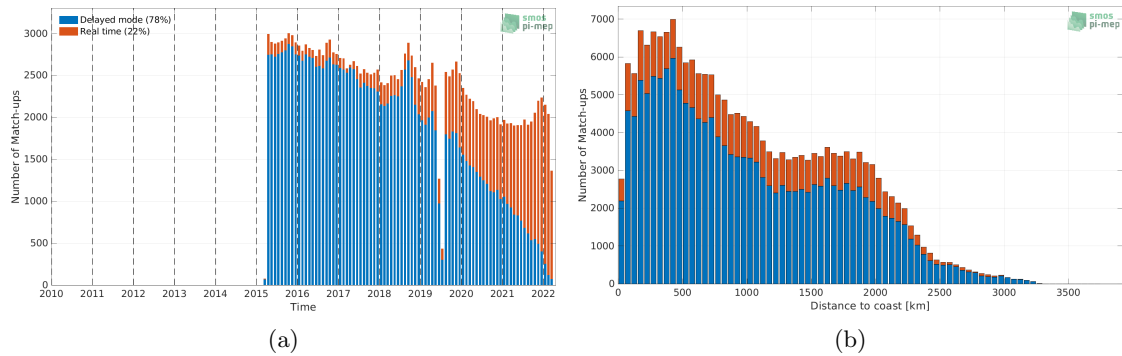
Figure 1: Number of match-ups between Argo and SMAP SSS L3 v4 - 8-Day running (RSS) SSS as a function of time (a) and as function of the distance to coast (b) over the Tropical Pacific Ocean Pi-MEP region and for the full satellite product period.
