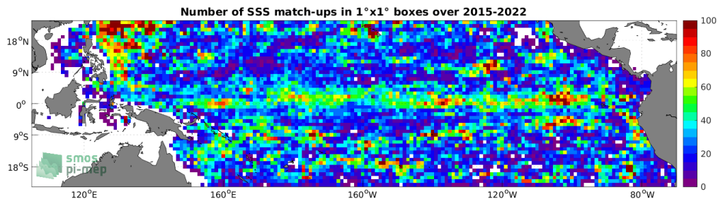
Figure 4: Number of SSS match-ups between Argo SSS and the SMAP SSS L3 v4 - 8-Day running (RSS) SSS product for the Tropical Pacific Ocean Pi-MEP region over 1^\circ \times 1^\circ boxes and for the full satellite product period.
