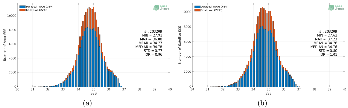
Figure 2: Histograms of SSS from Argo (a) and SMAP SSS L3 v4 - 8-Day running (RSS) (b) considering all match-up pairs per bins of 0.1 over the Tropical Pacific Ocean Pi-MEP region and for the full satellite product period.
