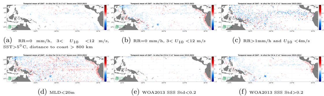
Figure 12: Temporal mean gridded over spatial boxes of size 1^\circ \times 1^\circ of \Delta SSS (SMAP SSS L3 v4 - 8-Day running (RSS) - Argo) for 6 different subdatasets corresponding to:RR=0 mm/h, 3 < U_{10} < 12 m/s, SST > 5^\circ C , distance to coast > 800 km (a), RR=0 mm/h, 3 < U_{10} < 12 m/s (b), RR >1 mm/h and U_{10} < 4 m/s (c),MLD <20 m (d),WOA2013 SSS Std <0.2 (e),WOA2013 SSS Std >0.2 (f).
