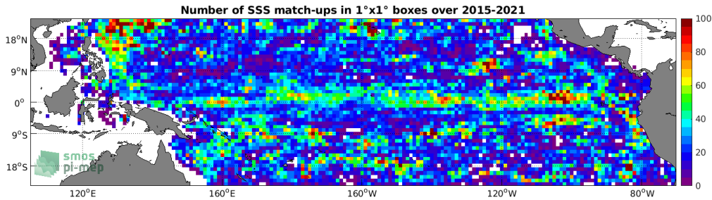
Figure 4: Number of SSS match-ups between Argo SSS and the SMAP SSS L3 v4 - 8-Day running (RSS) SSS product for the Tropical Pacific Ocean Pi-MEP region over 1^\circ \times 1^\circ boxes and for the full satellite product period.
