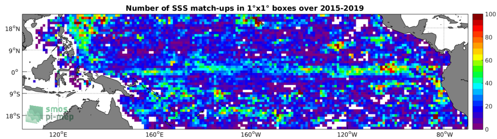
Figure 4: Number of SSS match-ups between Argo SSS and the SMAP-L3-RSS-V4-8DAY-RUNNING SSS product for the Tropical Pacific Ocean Pi-MEP region over 1^\circ \times 1^\circ boxes and for the full satellite product period.
