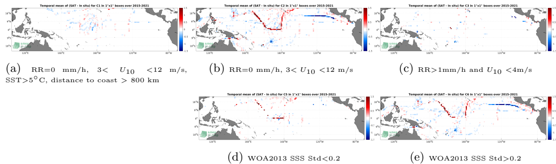
Figure 12: Temporal mean gridded over spatial boxes of size 1^\circ \times 1^\circ of \Delta\text{SSS} (SMAP SSS L3 v4 - Monthly (RSS) - TSG (SAMOS)) for 5 different subdatasets corresponding to:RR=0 mm/h, 3 < U_{10} < 12 m/s, SST >5^\circ\text{C} , distance to coast > 800 km (a), RR=0 mm/h, 3 < U_{10} < 12 m/s (b), RR >1 mm/h and U_{10} < 4 m/s (c), WOA2013 SSS Std <0.2 (d), WOA2013 SSS Std >0.2 (e).
