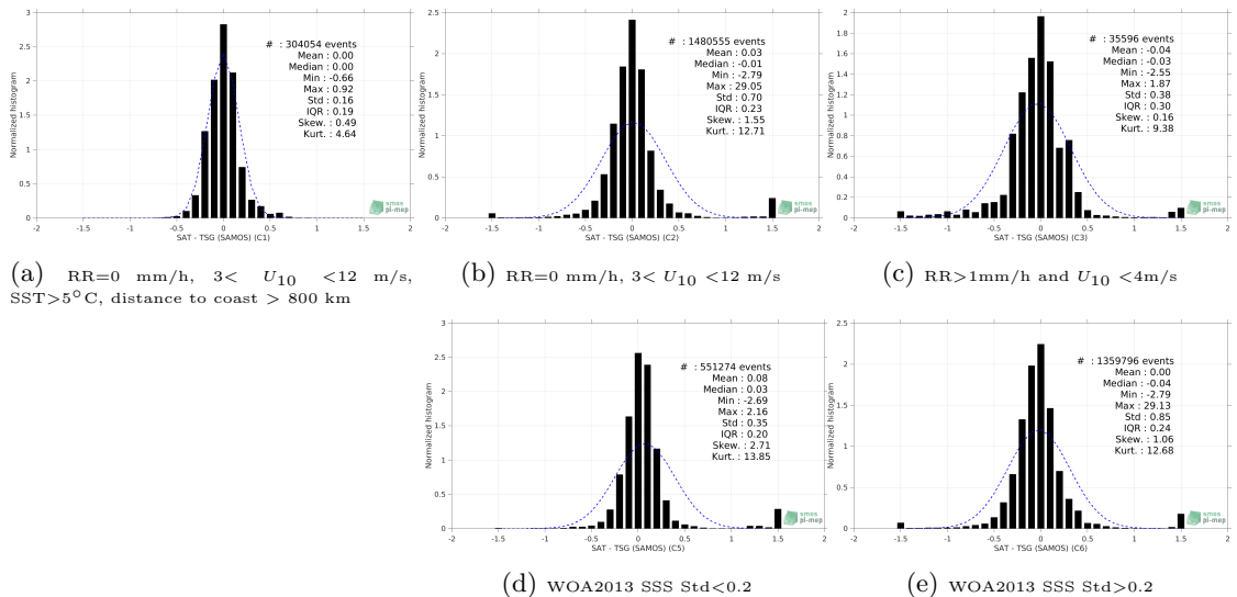
Figure 13: Normalized histogram of ΔSSS (SMAP SSS L3 v4 - Monthly (RSS) - TSG (SAMOS)) for 5 different subdatasets corresponding to: RR=0 mm/h, 3 < U 10 < 12 m/s, SST>5°C, distance to coast > 800 km (a), RR=0 mm/h, 3 < U 10 < 12 m/s (b), RR>1mm/h and U 10 < 4m/s (c), WOA2013 SSS Std<0.2 (d), WOA2013 SSS Std>0.2 (e).
