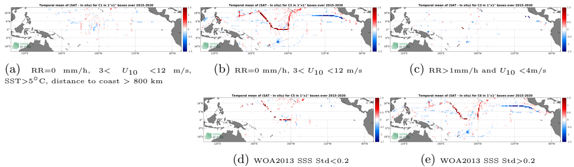
Figure 12: Temporal mean gridded over spatial boxes of size 1°x1° of ΔSSS (SMAP SSS L3 v4 - Monthly (RSS) - TSG (SAMOS)) for 5 different subdatasets corresponding to:RR=0 mm/h, 3 < U 10 < 12 m/s, SST>5°C, distance to coast > 800 km (a), RR=0 mm/h, 3 < U 10 < 12 m/s (b), RR>1mm/h and U 10 < 4m/s (c), WOA2013 SSS Std<0.2 (d), WOA2013 SSS Std>0.2 (e).
