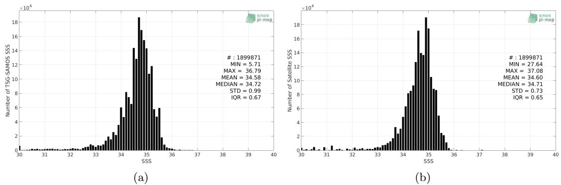
Figure 2: Histograms of SSS from TSG-SAMOS (a) and SMAP-L3-RSS-V4-MONTHLY (b) considering all match-up pairs per bins of 0.1 over the Tropical Pacific Ocean Pi-MEP region and for the full satellite product period.
