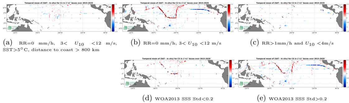
Figure 12: Temporal mean gridded over spatial boxes of size 1°x1° of \Delta SSS (SMAP-L3-RSS-V4-MONTHLY - TSG-SAMOS) for 5 different subdatasets corresponding to:RR=0 mm/h, 3< U_{10} <12 m/s, SST>5°C, distance to coast > 800 km (a), RR=0 mm/h, 3< U_{10} <12 m/s (b), RR>1mm/h and U_{10} <4m/s (c), WOA2013 SSS Std<0.2 (d), WOA2013 SSS Std>0.2 (e).
