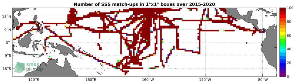
Figure 4: Number of SSS match-ups between TSG-SAMOS SSS and the SMAP-L3-RSS-V4-MONTHLY SSS product for the Tropical Pacific Ocean Pi-MEP region over 1^\circ \times 1^\circ boxes and for the full satellite product period.
