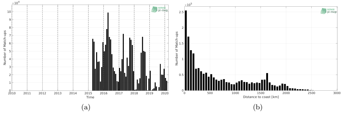
Figure 1: Number of match-ups between TSG-SAMOS and SMAP-L3-RSS-V4-MONTHLY SSS as a function of time (a) and as function of the distance to coast (b) over the Tropical Pacific Ocean Pi-MEP region and for the full satellite product period.
