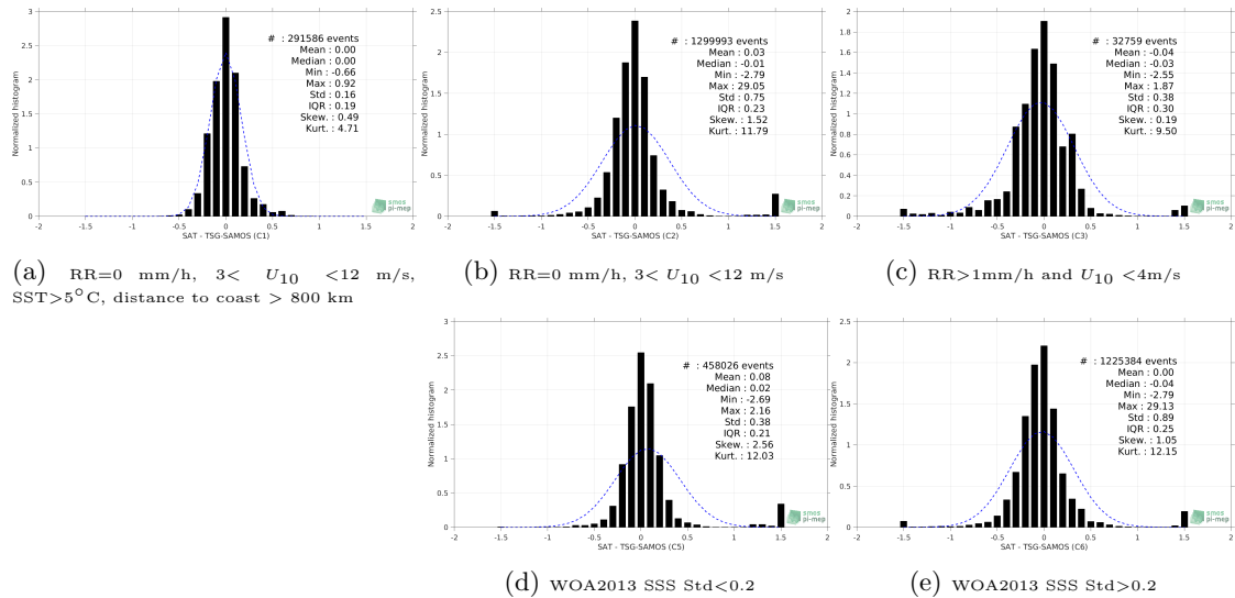
Figure 13: Normalized histogram of \Delta SSS (SMAP-L3-RSS-V4-MONTHLY - TSG-SAMOS) for 5 different subdatasets corresponding to: RR=0 mm/h, 3 < U_{10} < 12 m/s, SST >5^\circ C, distance to coast > 800 km (a), RR=0 mm/h, 3 < U_{10} < 12 m/s (b), RR >1 mm/h and U_{10} < 4 m/s (c), WOA2013 SSS Std <0.2 (d), WOA2013 SSS Std >0.2 (e).
