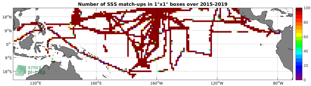
Figure 4: Number of SSS match-ups between TSG-SAMOS SSS and the SMAP-L3-RSS-V4-MONTHLY SSS product for the Tropical Pacific Ocean Pi-MEP region over 1°x1° boxes and for the full satellite product period.
