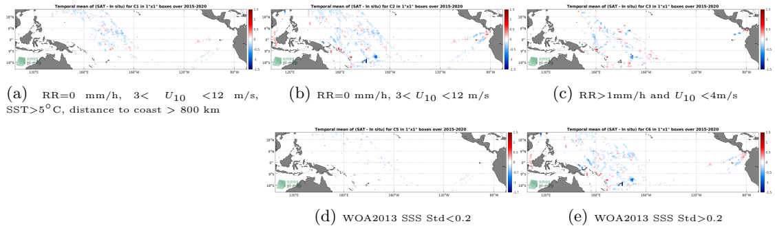
Figure 12: Temporal mean gridded over spatial boxes of size 1°x1° of ΔSSS (SMAP SSS L3 v4 - Monthly (RSS) - TSG (LEGOS-DM)) for 5 different subdatasets corresponding to:RR=0 mm/h, 3 < U 10 < 12 m/s, SST > 5°C, distance to coast > 800 km (a), RR=0 mm/h, 3 < U 10 < 12 m/s (b), RR > 1mm/h and U 10 < 4m/s (c), WOA2013 SSS Std < 0.2 (d), WOA2013 SSS Std > 0.2 (e).
