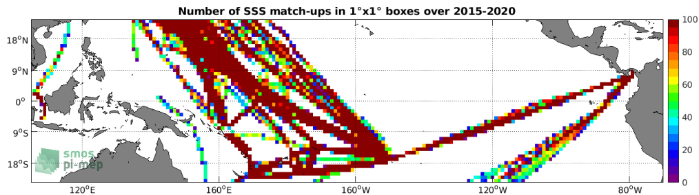
Figure 4: Number of SSS match-ups between TSG (LEGOS-DM) SSS and the SMAP SSS L3 v4 - Monthly (RSS) SSS product for the Tropical Pacific Ocean Pi-MEP region over 1^\circ \times 1^\circ boxes and for the full satellite product period.
