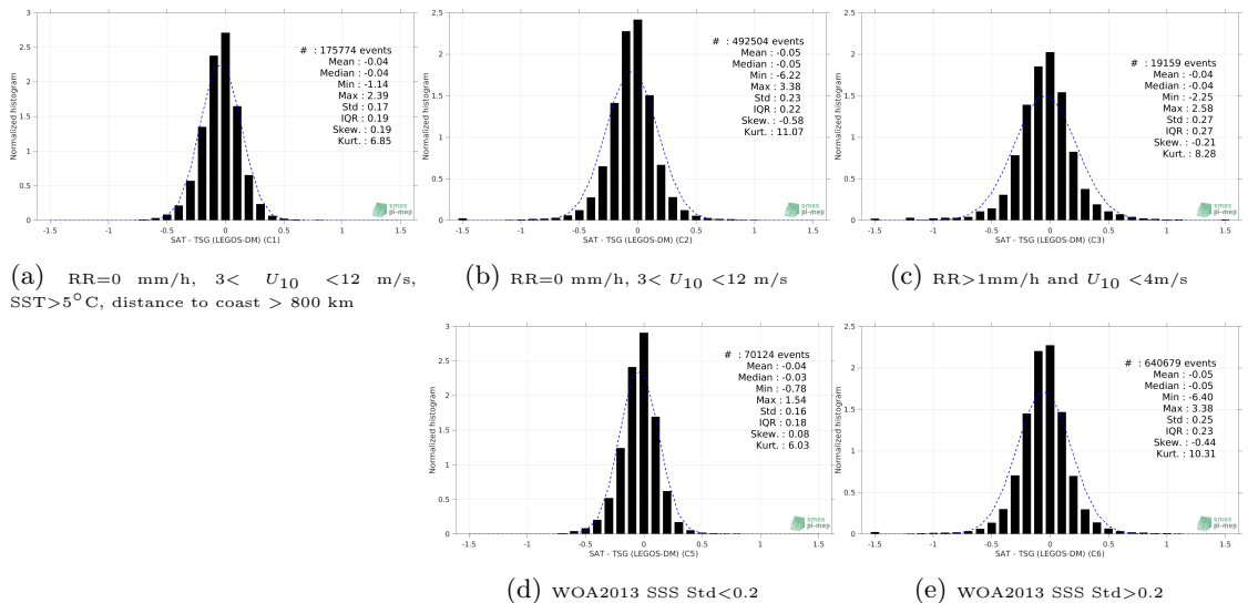
Figure 13: Normalized histogram of ΔSSS (SMAP SSS L3 v4 - Monthly (RSS) - TSG (LEGOS-DM)) for 5 different subdatasets corresponding to: RR=0 mm/h, 3 < U 10 < 12 m/s, SST > 5°C, distance to coast > 800 km (a), RR=0 mm/h, 3 < U 10 < 12 m/s (b), RR > 1mm/h and U 10 < 4m/s (c), WOA2013 SSS Std < 0.2 (d), WOA2013 SSS Std > 0.2 (e).
