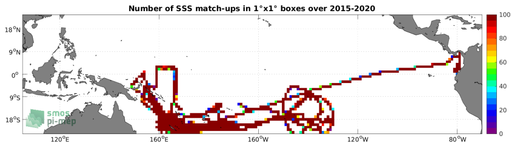
Figure 4: Number of SSS match-ups between TSG (GOSUD-Research-vessel) SSS and the SMAP SSS L3 v4 - Monthly (RSS) SSS product for the Tropical Pacific Ocean Pi-MEP region over 1^\circ \times 1^\circ boxes and for the full satellite product period.
