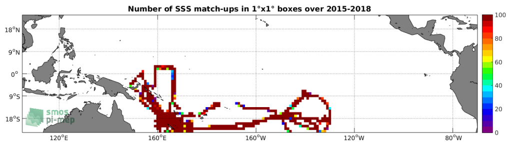
Figure 4: Number of SSS match-ups between TSG-GOSUD-Research-vessel SSS and the SMAP-L3-RSS-V4-MONTHLY SSS product for the Tropical Pacific Ocean Pi-MEP region over 1^\circ \times 1^\circ boxes and for the full satellite product period.
