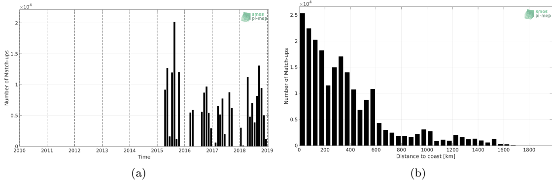
Figure 1: Number of match-ups between TSG-GOSUD-Research-vessel and SMAP-L3-RSS-V4-MONTHLY SSS as a function of time (a) and as function of the distance to coast (b) over the Tropical Pacific Ocean Pi-MEP region and for the full satellite product period.
