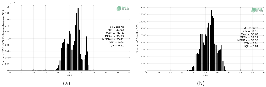
Figure 2: Histograms of SSS from TSG-GOSUD-Research-vessel (a) and SMAP-L3-RSS-V4-MONTHLY (b) considering all match-up pairs per bins of 0.1 over the Tropical Pacific Ocean Pi-MEP region and for the full satellite product period.
