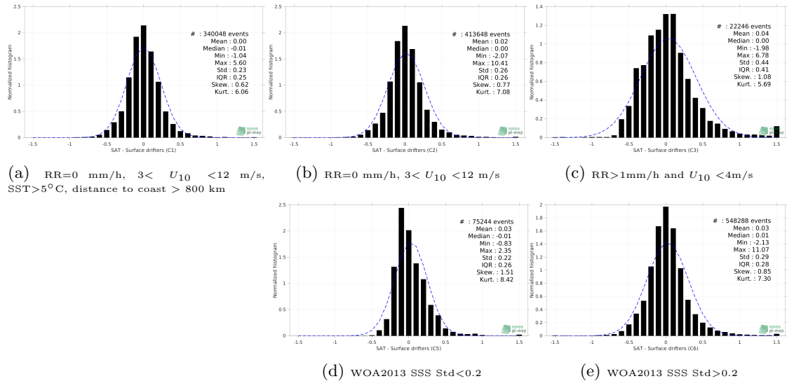
Figure 12: Normalized histogram of \Delta SSS (SMAP SSS L3 v4 - Monthly (RSS) - Surface drifters) for 5 different subdatasets corresponding to: RR=0 mm/h, 3 < U_{10} < 12 m/s, SST > 5^\circ C , distance to coast > 800 km (a), RR=0 mm/h, 3 < U_{10} < 12 m/s (b), RR>1mm/h and U_{10} < 4 m/s (c), WOA2013 SSS Std<0.2 (d), WOA2013 SSS Std>0.2 (e).
