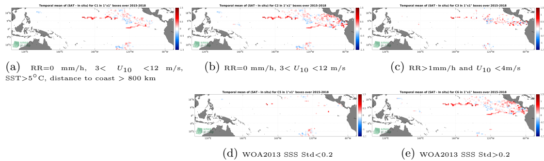
Figure 11: Temporal mean gridded over spatial boxes of size 1^\circ \times 1^\circ of \Delta SSS (SMAP SSS L3 v4 - Monthly (RSS) - Surface drifters) for 5 different subdatasets corresponding to:RR=0 mm/h, 3 < U_{10} < 12 m/s, SST > 5^\circ C , distance to coast > 800 km (a), RR=0 mm/h, 3 < U_{10} < 12 m/s (b), RR>1mm/h and U_{10} < 4 m/s (c), WOA2013 SSS Std<0.2 (d), WOA2013 SSS Std>0.2 (e).
