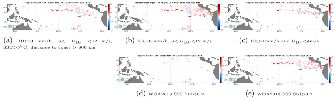
Figure 11: Temporal mean gridded over spatial boxes of size 1^\circ \times 1^\circ of \Delta SSS (SMAP SSS L3 v4 - Monthly (RSS) - Surface drifters) for 5 different subdatasets corresponding to:RR=0 mm/h, 3 < U_{10} < 12 m/s, SST > 5^\circ C , distance to coast > 800 km (a), RR=0 mm/h, 3 < U_{10} < 12 m/s (b), RR>1mm/h and U_{10} < 4 m/s (c), WOA2013 SSS Std<0.2 (d), WOA2013 SSS Std>0.2 (e).
