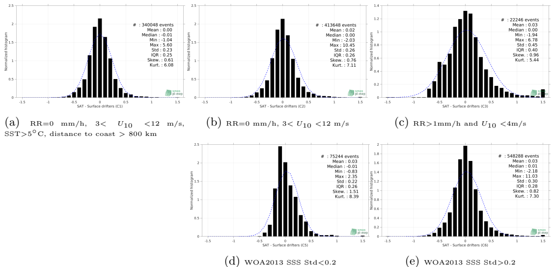
Figure 12: Normalized histogram of ΔSSS (SMAP SSS L3 v4 - Monthly (RSS) - Surface drifters) for 5 different subdatasets corresponding to: RR=0 mm/h, 3 < U 10 < 12 m/s, SST>5°C, distance to coast > 800 km (a), RR=0 mm/h, 3 < U 10 < 12 m/s (b), RR>1mm/h and U 10 < 4m/s (c), WOA2013 SSS Std<0.2 (d), WOA2013 SSS Std>0.2 (e).
