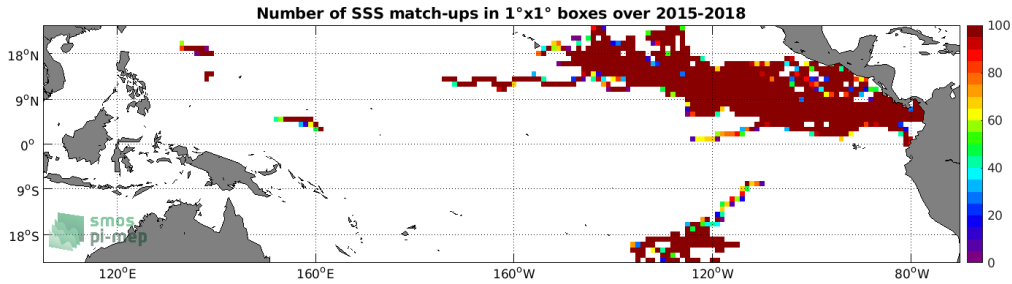
Figure 3: Number of SSS match-ups between Surface drifters SSS and the SMAP SSS L3 v4 - Monthly (RSS) SSS product for the Tropical Pacific Ocean Pi-MEP region over 1^\circ \times 1^\circ boxes and for the full satellite product period.
