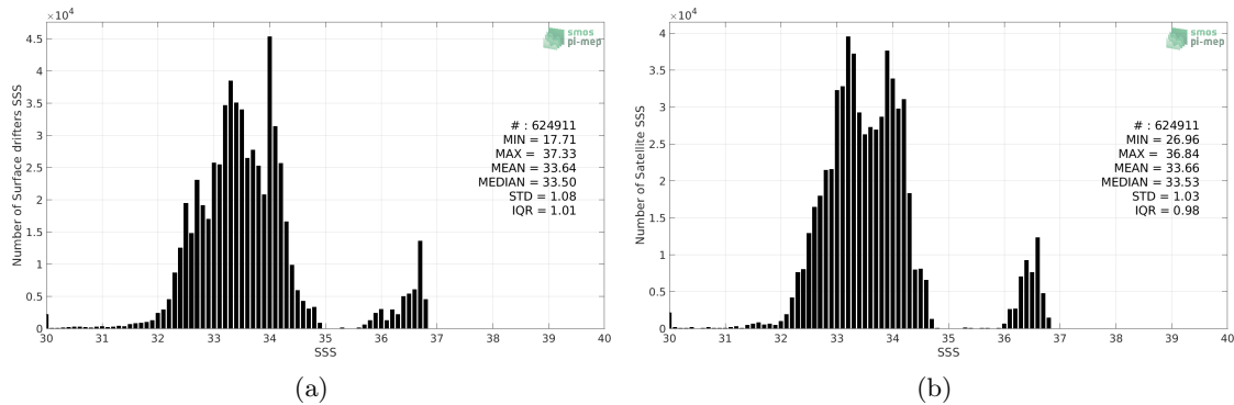
Figure 2: Histograms of SSS from Surface drifters (a) and SMAP SSS L3 v4 - Monthly (RSS) (b) considering all match-up pairs per bins of 0.1 over the Tropical Pacific Ocean Pi-MEP region and for the full satellite product period.
