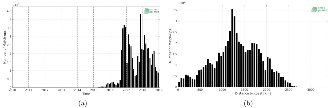
Figure 1: Number of match-ups between Surface drifters and SMAP SSS L3 v4 - Monthly (RSS) SSS as a function of time (a) and as function of the distance to coast (b) over the Tropical Pacific Ocean Pi-MEP region and for the full satellite product period.
