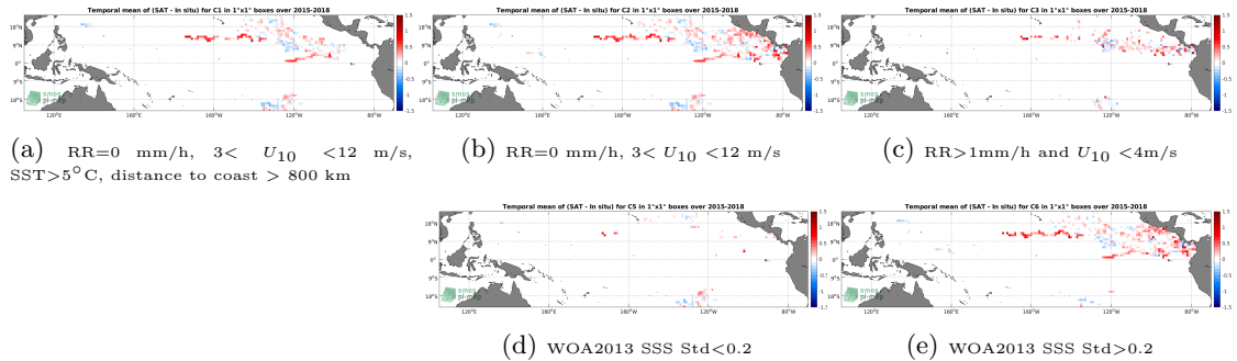
Figure 11: Temporal mean gridded over spatial boxes of size 1°x1° of ΔSSS (SMAP SSS L3 v4 - Monthly (RSS) - Surface drifters) for 5 different subdatasets corresponding to:RR=0 mm/h, 3 < U 10 < 12 m/s, SST>5°C, distance to coast > 800 km (a), RR=0 mm/h, 3 < U 10 < 12 m/s (b), RR>1mm/h and U 10 < 4m/s (c), WOA2013 SSS Std<0.2 (d), WOA2013 SSS Std>0.2 (e).
