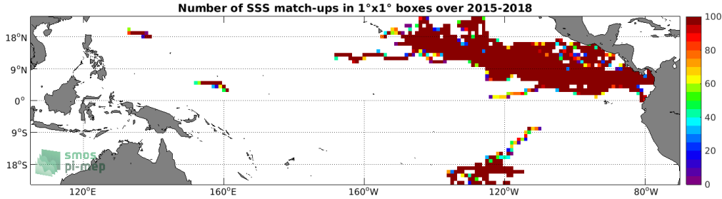
Figure 3: Number of SSS match-ups between Surface drifters SSS and the SMAP SSS L3 v4 - Monthly (RSS) SSS product for the Tropical Pacific Ocean Pi-MEP region over 1^\circ \times 1^\circ boxes and for the full satellite product period.
