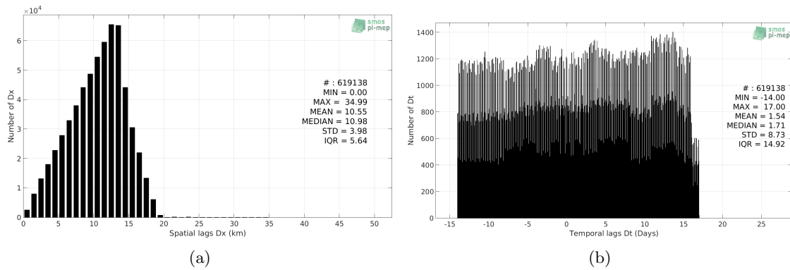
Figure 4: Histograms of the spatial (a) and temporal (b) lags between the time of the Surface drifters measurements and the date of the corresponding SMAP-L3-RSS-V4-MONTHLY SSS product.
