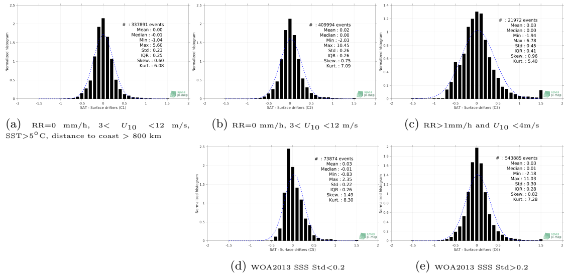
Figure 12: Normalized histogram of \Delta SSS (SMAP-L3-RSS-V4-MONTHLY - Surface drifters) for 5 different subdatasets corresponding to: RR=0 mm/h, 3 < U_{10} < 12 m/s, SST >5^\circ\text{C} , distance to coast > 800 km (a), RR=0 mm/h, 3 < U_{10} < 12 m/s (b), RR >1 mm/h and U_{10} < 4 m/s (c), WOA2013 SSS Std <0.2 (d), WOA2013 SSS Std >0.2 (e).
