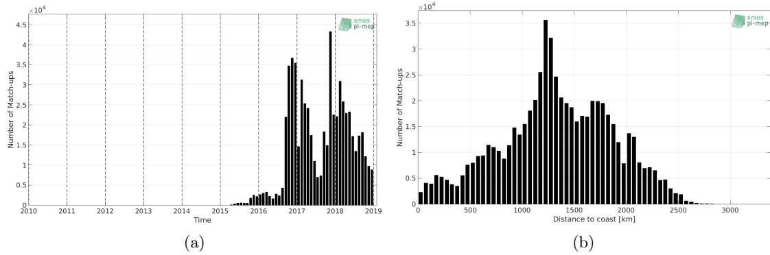
Figure 1: Number of match-ups between Surface drifters and SMAP-L3-RSS-V4-MONTHLY SSS as a function of time (a) and as function of the distance to coast (b) over the Tropical Pacific Ocean Pi-MEP region and for the full satellite product period.
