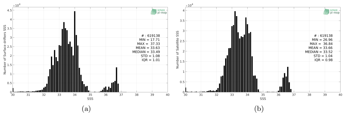
Figure 2: Histograms of SSS from Surface drifters (a) and SMAP-L3-RSS-V4-MONTHLY (b) considering all match-up pairs per bins of 0.1 over the Tropical Pacific Ocean Pi-MEP region and for the full satellite product period.
