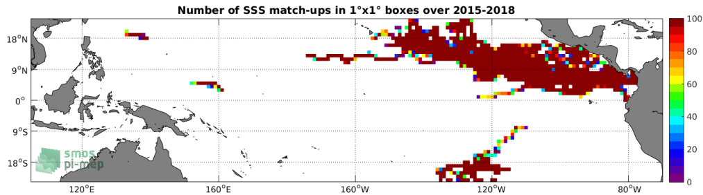
Figure 3: Number of SSS match-ups between Surface drifters SSS and the SMAP-L3-RSS-V4-MONTHLY SSS product for the Tropical Pacific Ocean Pi-MEP region over 1^\circ \times 1^\circ boxes and for the full satellite product period.
