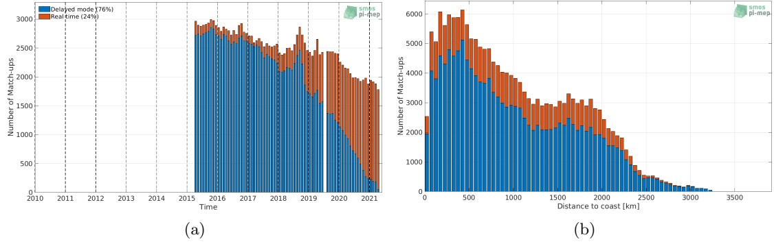
Figure 1: Number of match-ups between Argo and SMAP SSS L3 v4 - Monthly (RSS) SSS as a function of time (a) and as function of the distance to coast (b) over the Tropical Pacific Ocean Pi-MEP region and for the full satellite product period.
