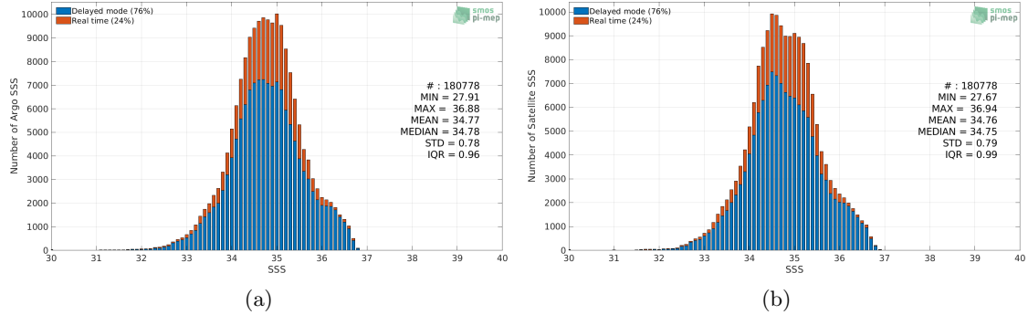
Figure 2: Histograms of SSS from Argo (a) and SMAP SSS L3 v4 - Monthly (RSS) (b) considering all match-up pairs per bins of 0.1 over the Tropical Pacific Ocean Pi-MEP region and for the full satellite product period.
