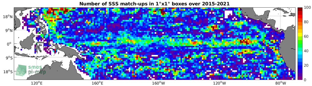
Figure 4: Number of SSS match-ups between Argo SSS and the SMAP SSS L3 v4 - Monthly (RSS) SSS product for the Tropical Pacific Ocean Pi-MEP region over 1^\circ \times 1^\circ boxes and for the full satellite product period.
