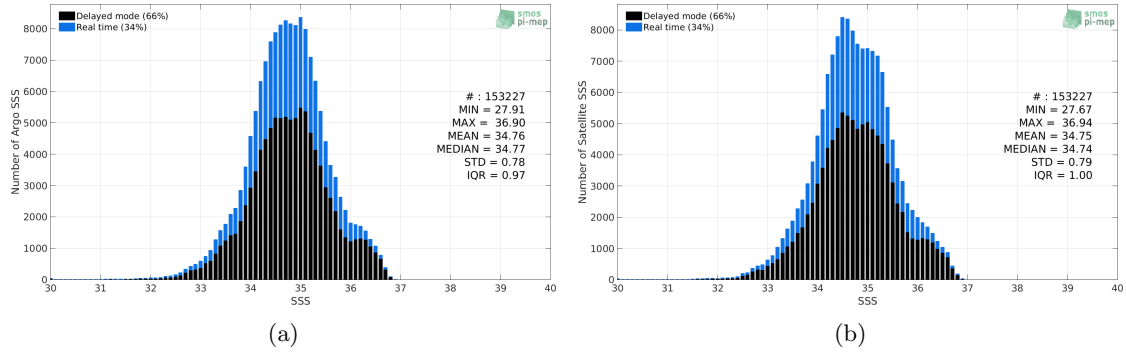
Figure 2: Histograms of SSS from Argo (a) and SMAP-L3-RSS-V4-MONTHLY (b) considering all match-up pairs per bins of 0.1 over the Tropical Pacific Ocean Pi-MEP region and for the full satellite product period.
