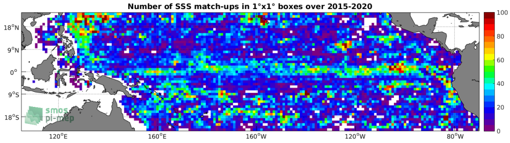
Figure 4: Number of SSS match-ups between Argo SSS and the SMAP-L3-RSS-V4-MONTHLY SSS product for the Tropical Pacific Ocean Pi-MEP region over 1^\circ \times 1^\circ boxes and for the full satellite product period.
