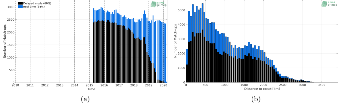
Figure 1: Number of match-ups between Argo and SMAP-L3-RSS-V4-MONTHLY SSS as a function of time (a) and as function of the distance to coast (b) over the Tropical Pacific Ocean Pi-MEP region and for the full satellite product period.
