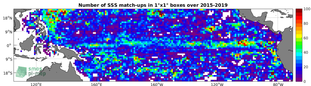
Figure 4: Number of SSS match-ups between Argo SSS and the SMAP-L3-RSS-V4-MONTHLY SSS product for the Tropical Pacific Ocean Pi-MEP region over 1^\circ \times 1^\circ boxes and for the full satellite product period.
