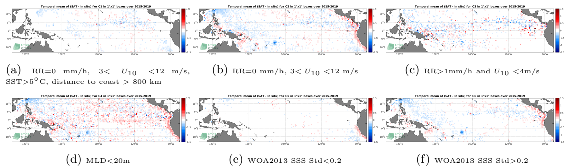
Figure 12: Temporal mean gridded over spatial boxes of size 1^\circ \times 1^\circ of \Delta SSS (SMAP-L3-RSS-V4-MONTHLY - Argo) for 6 different subdatasets corresponding to:RR=0 mm/h, 3 < U_{10} < 12 m/s, SST >5^\circ C, distance to coast > 800 km (a), RR=0 mm/h, 3 < U_{10} < 12 m/s (b), RR >1 mm/h and U_{10} < 4 m/s (c),MLD <20 m (d),WOA2013 SSS Std <0.2 (e),WOA2013 SSS Std >0.2 (f).
