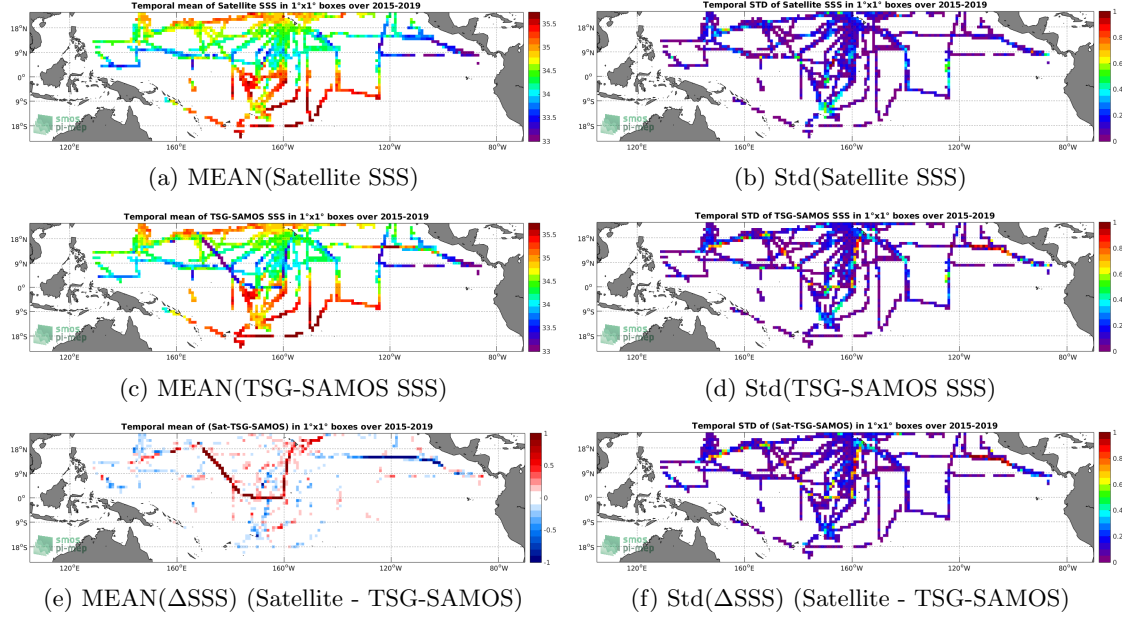
Figure 6: Temporal mean (left) and Std (right) of SSS from SMAP-L3-RSS-V3-8DAY-RUNNING-70KM (top), TSG-SAMOS (middle), and of \Delta SSS (Satellite - TSG-SAMOS). Only match-up pairs are used to generate these maps.
