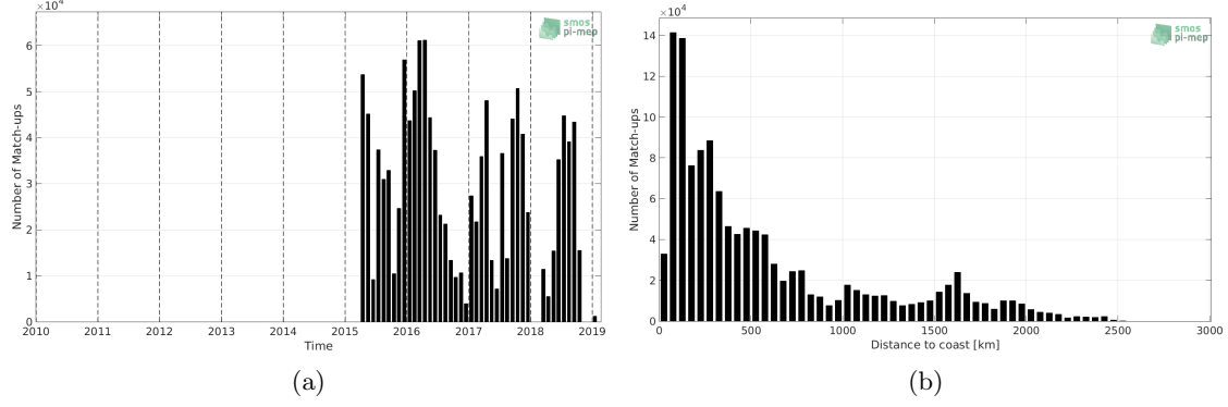
Figure 1: Number of match-ups between TSG-SAMOS and SMAP-L3-RSS-V3-8DAY-RUNNING-70KM SSS as a function of time (a) and as function of the distance to coast (b) over the Tropical Pacific Ocean Pi-MEP region and for the full satellite product period.
