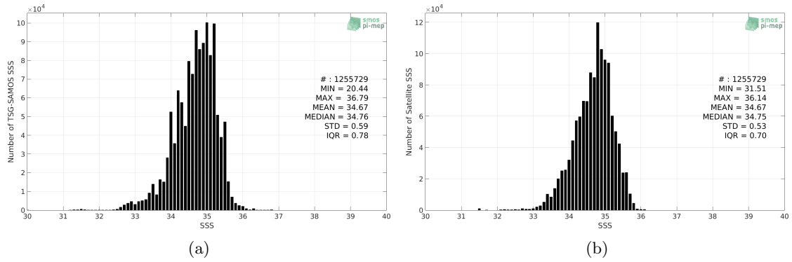
Figure 2: Histograms of SSS from TSG-SAMOS (a) and SMAP-L3-RSS-V3-8DAY-RUNNING-70KM (b) considering all match-up pairs per bins of 0.1 over the Tropical Pacific Ocean Pi-MEP region and for the full satellite product period.
