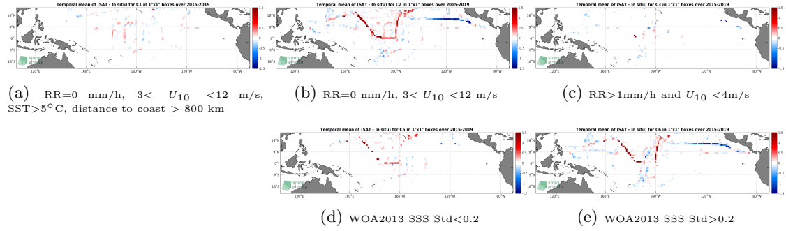
Figure 12: Temporal mean gridded over spatial boxes of size 1^\circ \times 1^\circ of \Delta SSS (SMAP-L3-RSS-V3-8DAY-RUNNING-70KM - TSG-SAMOS) for 5 different subdatasets corresponding to: RR=0 mm/h, 3 < U_{10} < 12 m/s, SST > 5^\circ C , distance to coast > 800 km (a), RR=0 mm/h, 3 < U_{10} < 12 m/s (b), RR > 1 mm/h and U_{10} < 4 m/s (c), WOA2013 SSS Std < 0.2 (d), WOA2013 SSS Std > 0.2 (e).
