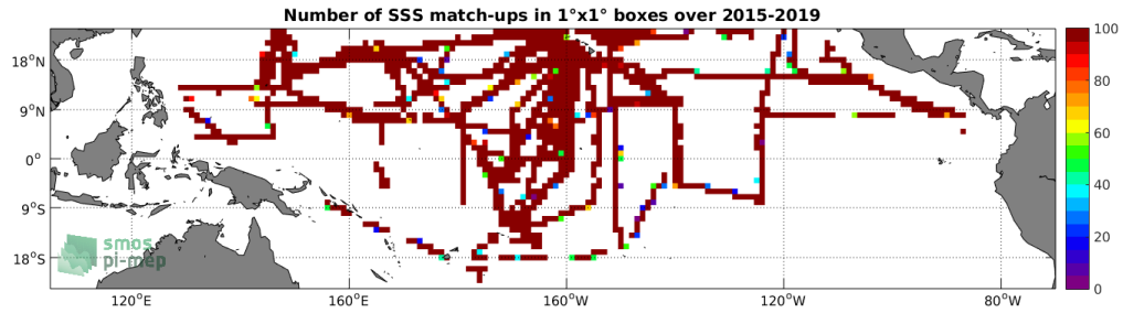
Figure 4: Number of SSS match-ups between TSG-SAMOS SSS and the SMAP-L3-RSS-V3-8DAY-RUNNING-70KM SSS product for the Tropical Pacific Ocean Pi-MEP region over 1°x1° boxes and for the full satellite product period.
