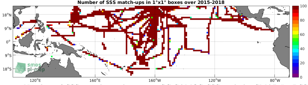
Figure 4: Number of SSS match-ups between TSG-SAMOS SSS and the SMAP-L3-RSS-V3-8DAY-RUNNING-70KM SSS product for the Tropical Pacific Ocean Pi-MEP region over 1^\circ \times 1^\circ boxes and for the full satellite product period.
