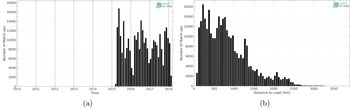
Figure 1: Number of match-ups between TSG-LEGOS-DM and SMAP-L3-RSS-V3-8DAY-RUNNING-70KM SSS as a function of time (a) and as function of the distance to coast (b) over the Tropical Pacific Ocean Pi-MEP region and for the full satellite product period.
