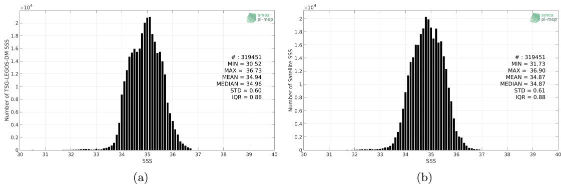
Figure 2: Histograms of SSS from TSG-LEGOS-DM (a) and SMAP-L3-RSS-V3-8DAY-RUNNING-70KM (b) considering all match-up pairs per bins of 0.1 over the Tropical Pacific Ocean Pi-MEP region and for the full satellite product period.
