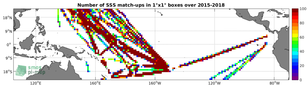
Figure 4: Number of SSS match-ups between TSG-LEGOS-DM SSS and the SMAP-L3-RSS-V3-8DAY-RUNNING-70KM SSS product for the Tropical Pacific Ocean Pi-MEP region over 1^\circ \times 1^\circ boxes and for the full satellite product period.
