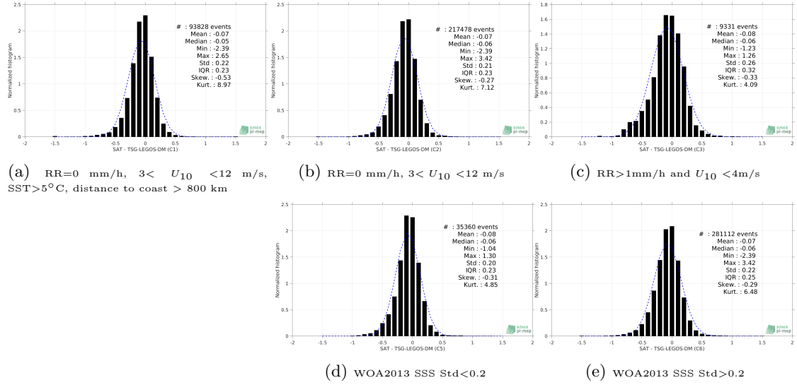
Figure 13: Normalized histogram of \Delta SSS (SMAP-L3-RSS-V3-8DAY-RUNNING-70KM - TSG-LEGOS-DM) for 5 different subdatasets corresponding to: RR=0 mm/h, 3 < U_{10} < 12 m/s, SST>5°C, distance to coast > 800 km (a), RR=0 mm/h, 3 < U_{10} < 12 m/s (b), RR>1mm/h and U_{10} < 4 m/s (c), WOA2013 SSS Std<0.2 (d), WOA2013 SSS Std>0.2 (e).
