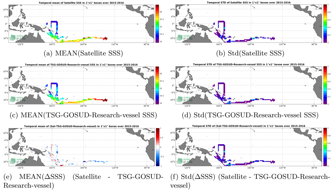
Figure 6: Temporal mean (left) and Std (right) of SSS from SMAP-L3-RSS-V3-8DAY-RUNNING-70KM (top), TSG-GOSUD-Research-vessel (middle), and of \Delta SSS (Satellite - TSG-GOSUD-Research-vessel). Only match-up pairs are used to generate these maps.
