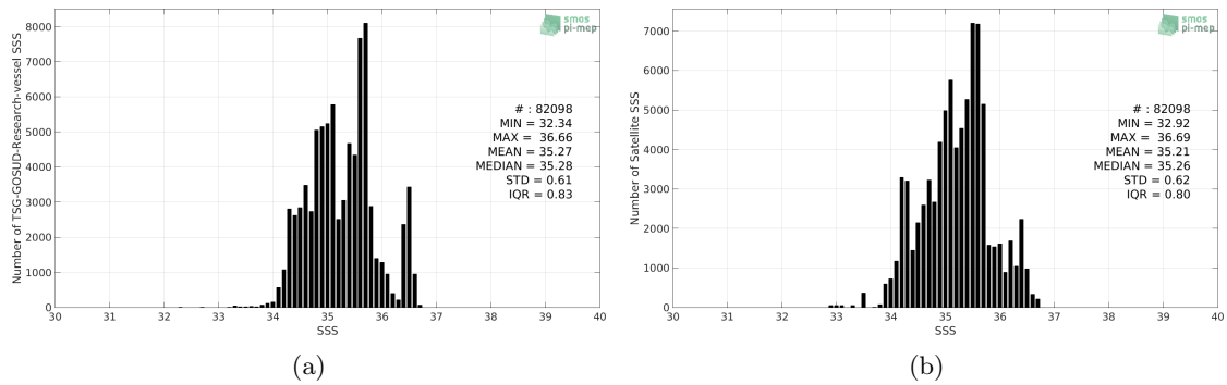
Figure 2: Histograms of SSS from TSG-GOSUD-Research-vessel (a) and SMAP-L3-RSS-V3-8DAY-RUNNING-70KM (b) considering all match-up pairs per bins of 0.1 over the Tropical Pacific Ocean Pi-MEP region and for the full satellite product period.
