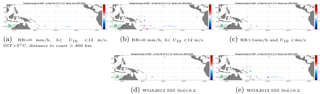
Figure 12: Temporal mean gridded over spatial boxes of size 1^\circ \times 1^\circ of \Delta SSS (SMAP-L3-RSS-V3-8DAY-RUNNING-70KM - TSG-GOSUD-Research-vessel) for 5 different subdatasets corresponding to:RR=0 mm/h, 3 < U_{10} < 12 m/s, SST > 5^\circ\text{C} , distance to coast > 800 km (a), RR=0 mm/h, 3 < U_{10} < 12 m/s (b), RR > 1 mm/h and U_{10} < 4 m/s (c), WOA2013 SSS Std < 0.2 (d), WOA2013 SSS Std > 0.2 (e).
