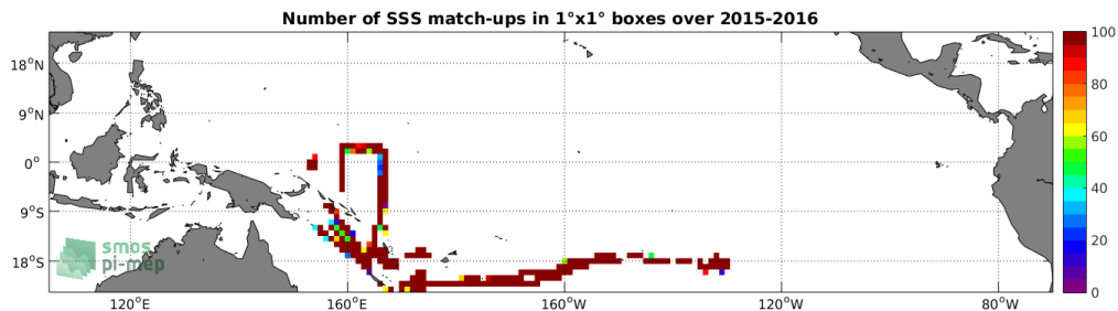
Figure 4: Number of SSS match-ups between TSG-GOSUD-Research-vessel SSS and the SMAP-L3-RSS-V3-8DAY-RUNNING-70KM SSS product for the Tropical Pacific Ocean Pi-MEP region over 1^\circ \times 1^\circ boxes and for the full satellite product period.
