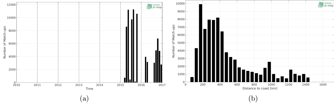
Figure 1: Number of match-ups between TSG-GOSUD-Research-vessel and SMAP-L3-RSS-V3-8DAY-RUNNING-70KM SSS as a function of time (a) and as function of the distance to coast (b) over the Tropical Pacific Ocean Pi-MEP region and for the full satellite product period.
