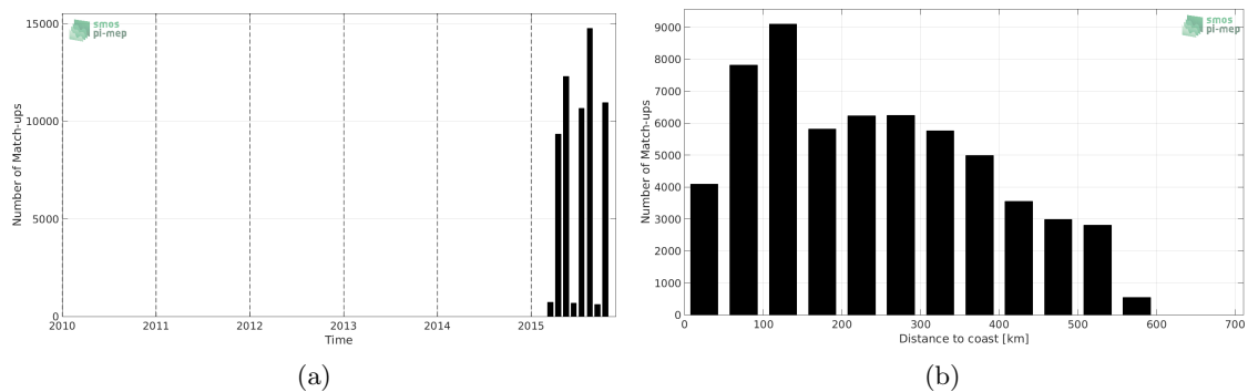
Figure 1: Number of match-ups between TSG-GOSUD-Research-vessel and SMAP-L3-RSS-V3-8DAY-RUNNING-70KM SSS as a function of time (a) and as function of the distance to coast (b) over the Tropical Pacific Ocean Pi-MEP region and for the full satellite product period.
