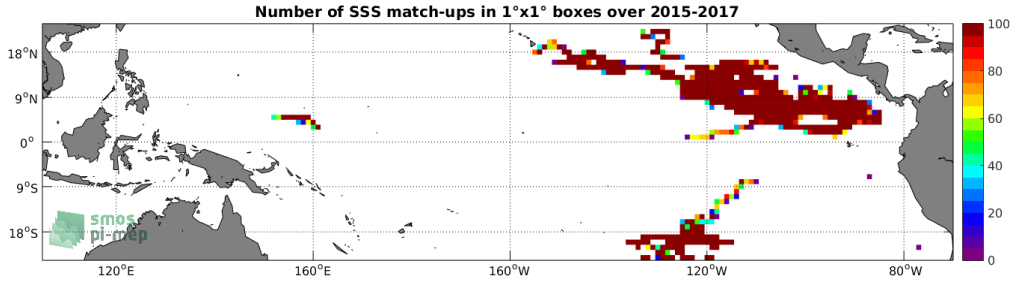
Figure 3: Number of SSS match-ups between Surface drifters SSS and the SMAP-L3-RSS-V3-8DAY-RUNNING-70KM SSS product for the Tropical Pacific Ocean Pi-MEP region over 1^\circ \times 1^\circ boxes and for the full satellite product period.
