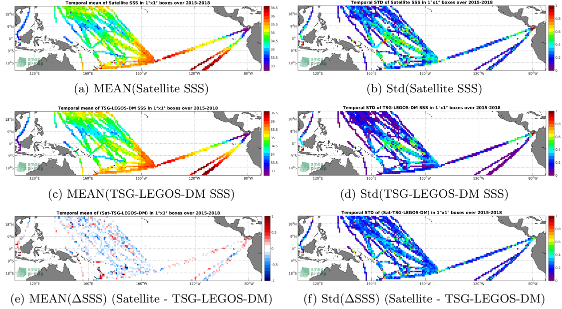
Figure 6: Temporal mean (left) and Std (right) of SSS from SMAP-L3-RSS-V3-8DAY-RUNNING-40KM (top), TSG-LEGOS-DM (middle), and of \Delta SSS (Satellite - TSG-LEGOS-DM). Only match-up pairs are used to generate these maps.
