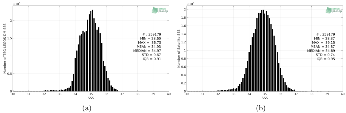
Figure 2: Histograms of SSS from TSG-LEGOS-DM (a) and SMAP-L3-RSS-V3-8DAY-RUNNING-40KM (b) considering all match-up pairs per bins of 0.1 over the Tropical Pacific Ocean Pi-MEP region and for the full satellite product period.
