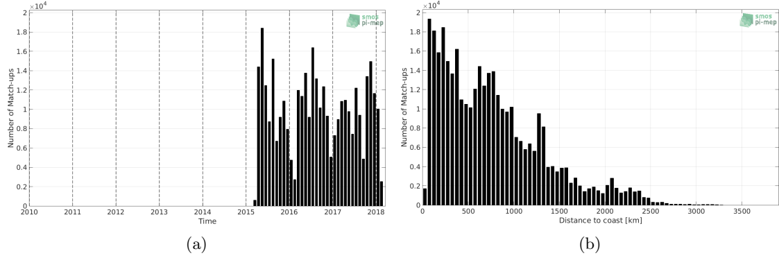
Figure 1: Number of match-ups between TSG-LEGOS-DM and SMAP-L3-RSS-V3-8DAY-RUNNING-40KM SSS as a function of time (a) and as function of the distance to coast (b) over the Tropical Pacific Ocean Pi-MEP region and for the full satellite product period.
