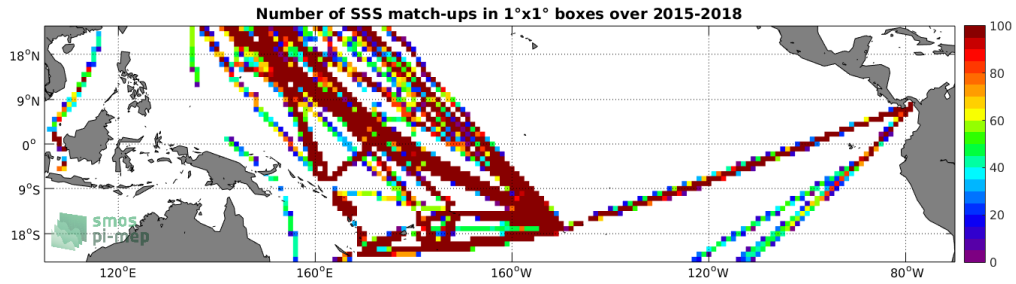
Figure 4: Number of SSS match-ups between TSG-LEGOS-DM SSS and the SMAP-L3-RSS-V3-8DAY-RUNNING-40KM SSS product for the Tropical Pacific Ocean Pi-MEP region over 1°x1° boxes and for the full satellite product period.
