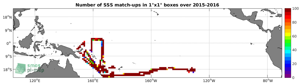
Figure 4: Number of SSS match-ups between TSG-GOSUD-Research-vessel SSS and the SMAP-L3-RSS-V3-8DAY-RUNNING-40KM SSS product for the Tropical Pacific Ocean Pi-MEP region over 1^\circ \times 1^\circ boxes and for the full satellite product period.
