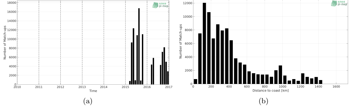
Figure 1: Number of match-ups between TSG-GOSUD-Research-vessel and SMAP-L3-RSS-V3-8DAY-RUNNING-40KM SSS as a function of time (a) and as function of the distance to coast (b) over the Tropical Pacific Ocean Pi-MEP region and for the full satellite product period.
