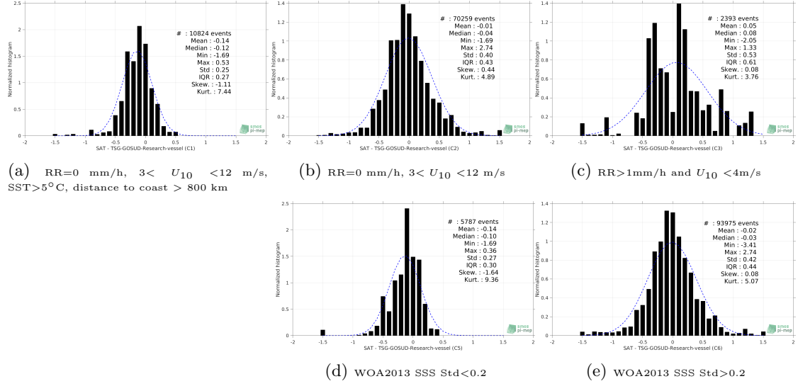
Figure 13: Normalized histogram of \Delta SSS (SMAP-L3-RSS-V3-8DAY-RUNNING-40KM - TSG-GOSUD-Research-vessel) for 5 different subdatasets corresponding to: RR=0 mm/h, 3 < U_{10} < 12 m/s, SST > 5^\circ\text{C} , distance to coast > 800 km (a), RR=0 mm/h, 3 < U_{10} < 12 m/s (b), RR > 1 mm/h and U_{10} < 4 m/s (c), WOA2013 SSS Std < 0.2 (d), WOA2013 SSS Std > 0.2 (e).
