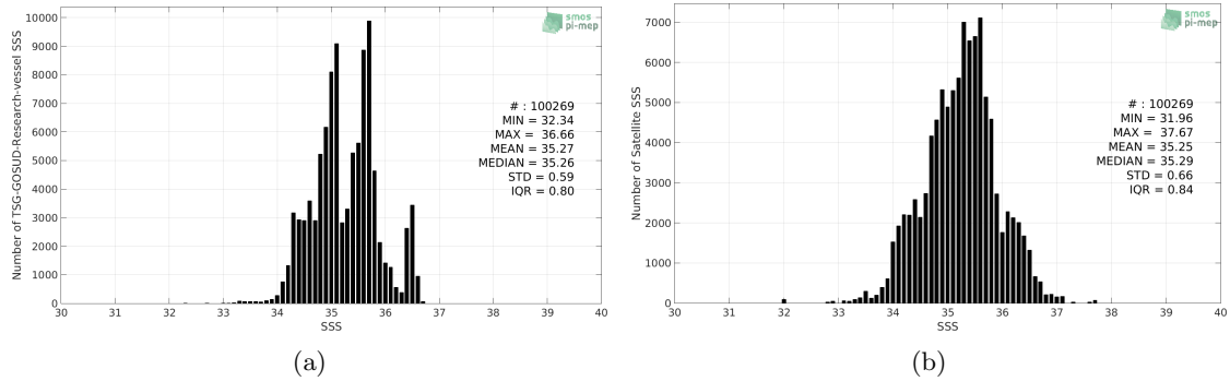
Figure 2: Histograms of SSS from TSG-GOSUD-Research-vessel (a) and SMAP-L3-RSS-V3-8DAY-RUNNING-40KM (b) considering all match-up pairs per bins of 0.1 over the Tropical Pacific Ocean Pi-MEP region and for the full satellite product period.
