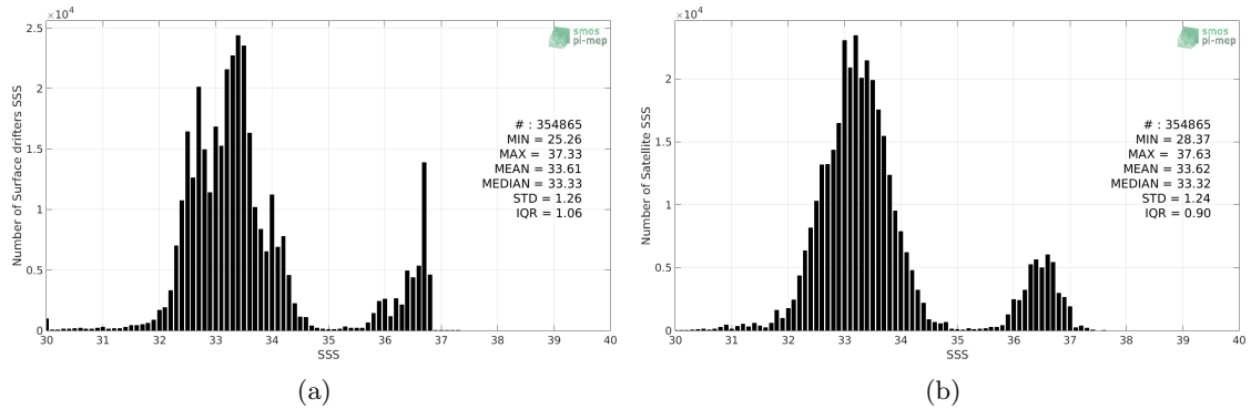
Figure 2: Histograms of SSS from Surface drifters (a) and SMAP-L3-RSS-V3-8DAY-RUNNING-40KM (b) considering all match-up pairs per bins of 0.1 over the Tropical Pacific Ocean Pi-MEP region and for the full satellite product period.
