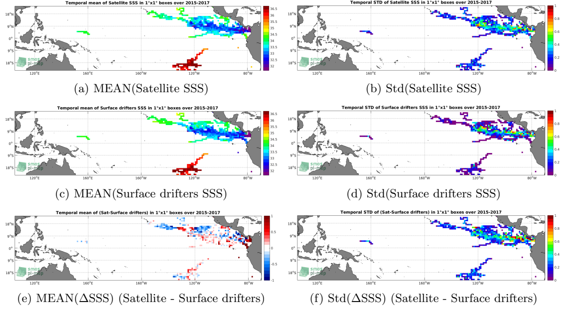
Figure 5: Temporal mean (left) and Std (right) of SSS from SMAP-L3-RSS-V3-8DAY-RUNNING-40KM (top), Surface drifters (middle), and of \Delta SSS (Satellite - Surface drifters). Only match-up pairs are used to generate these maps.
