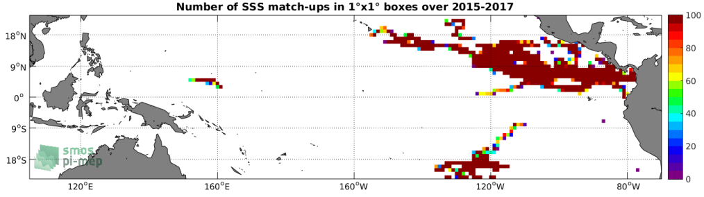
Figure 3: Number of SSS match-ups between Surface drifters SSS and the SMAP-L3-RSS-V3-8DAY-RUNNING-40KM SSS product for the Tropical Pacific Ocean Pi-MEP region over 1^\circ \times 1^\circ boxes and for the full satellite product period.
