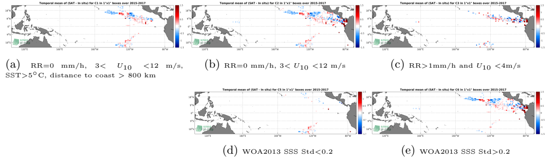
Figure 11: Temporal mean gridded over spatial boxes of size 1^\circ \times 1^\circ of \Delta SSS (SMAP-L3-RSS-V3-8DAY-RUNNING-40KM - Surface drifters) for 5 different subdatasets corresponding to: RR=0 mm/h, 3 < U_{10} < 12 m/s, SST > 5^\circ C , distance to coast > 800 km (a), RR=0 mm/h, 3 < U_{10} < 12 m/s (b), RR > 1 mm/h and U_{10} < 4 m/s (c), WOA2013 SSS Std < 0.2 (d), WOA2013 SSS Std > 0.2 (e).
