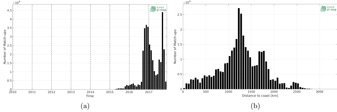
Figure 1: Number of match-ups between Surface drifters and SMAP-L3-RSS-V3-8DAY-RUNNING-40KM SSS as a function of time (a) and as function of the distance to coast (b) over the Tropical Pacific Ocean Pi-MEP region and for the full satellite product period.
