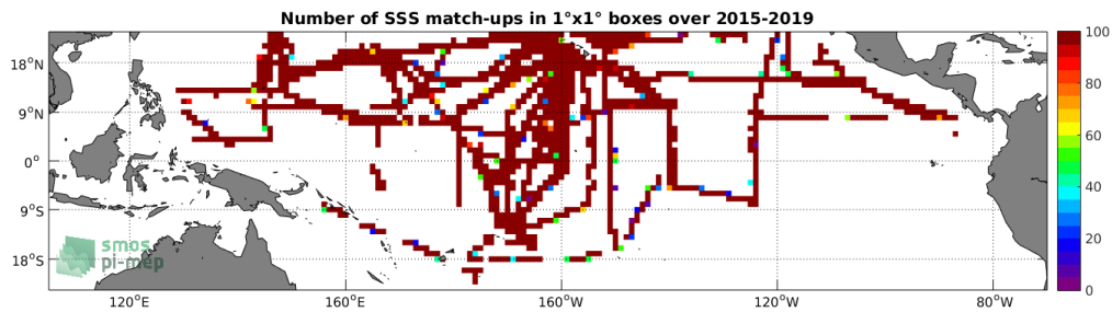
Figure 4: Number of SSS match-ups between TSG-SAMOS SSS and the SMAP-L3-RSS-V3-MONTHLY-70KM SSS product for the Tropical Pacific Ocean Pi-MEP region over 1^\circ \times 1^\circ boxes and for the full satellite product period.
