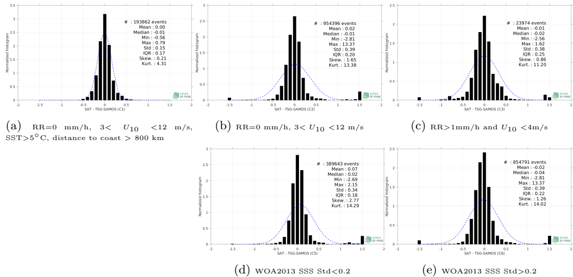
Figure 13: Normalized histogram of \Delta SSS (SMAP-L3-RSS-V3-MONTHLY-70KM - TSG-SAMOS) for 5 different subdatasets corresponding to: RR=0 mm/h, 3 < U_{10} < 12 m/s, SST >5^\circ C, distance to coast > 800 km (a), RR=0 mm/h, 3 < U_{10} < 12 m/s (b), RR >1 mm/h and U_{10} < 4 m/s (c), WOA2013 SSS Std <0.2 (d), WOA2013 SSS Std >0.2 (e).
