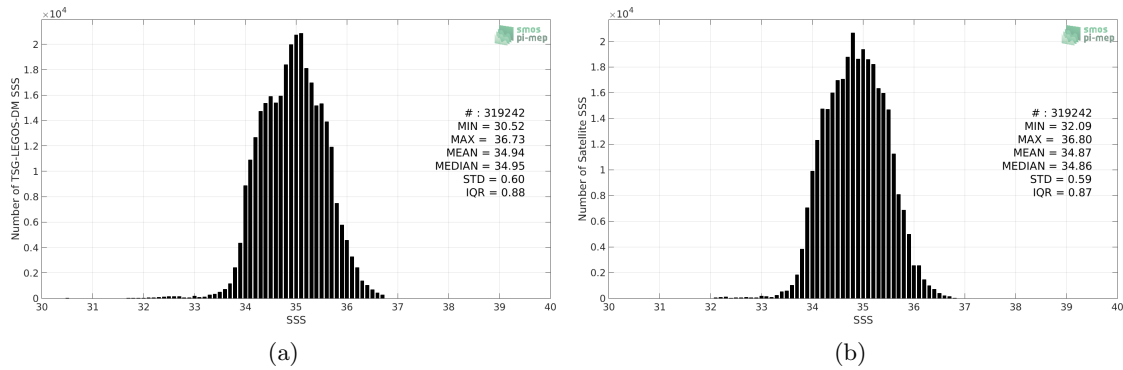
Figure 2: Histograms of SSS from TSG-LEGOS-DM (a) and SMAP-L3-RSS-V3-MONTHLY-70KM (b) considering all match-up pairs per bins of 0.1 over the Tropical Pacific Ocean Pi-MEP region and for the full satellite product period.
