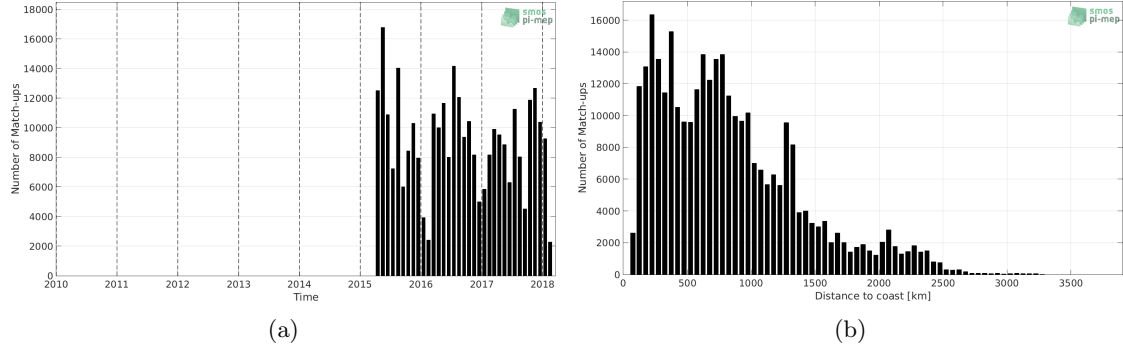
Figure 1: Number of match-ups between TSG-LEGOS-DM and SMAP-L3-RSS-V3-MONTHLY-70KM SSS as a function of time (a) and as function of the distance to coast (b) over the Tropical Pacific Ocean Pi-MEP region and for the full satellite product period.
