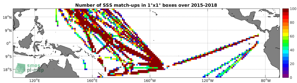
Figure 4: Number of SSS match-ups between TSG-LEGOS-DM SSS and the SMAP-L3-RSS-V3-MONTHLY-70KM SSS product for the Tropical Pacific Ocean Pi-MEP region over 1^\circ \times 1^\circ boxes and for the full satellite product period.
