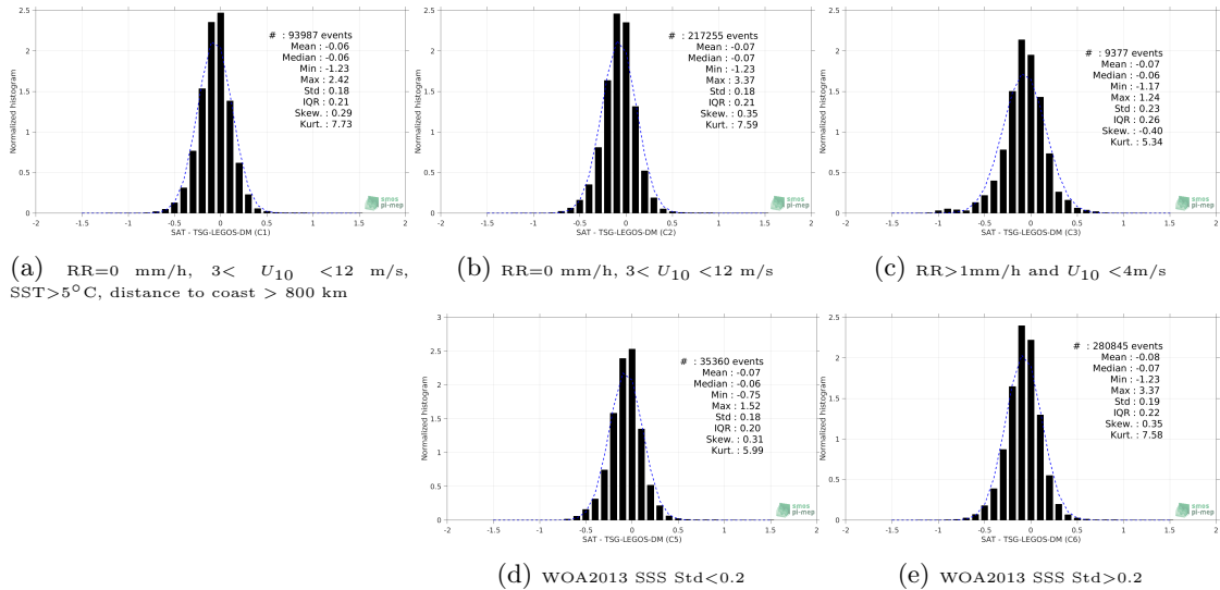
Figure 13: Normalized histogram of \Delta SSS (SMAP-L3-RSS-V3-MONTHLY-70KM - TSG-LEGOS-DM) for 5 different subdatasets corresponding to: RR=0 mm/h, 3 < U_{10} < 12 m/s, SST >5^\circ C, distance to coast > 800 km (a), RR=0 mm/h, 3 < U_{10} < 12 m/s (b), RR >1 mm/h and U_{10} < 4 m/s (c), WOA2013 SSS Std <0.2 (d), WOA2013 SSS Std >0.2 (e).
