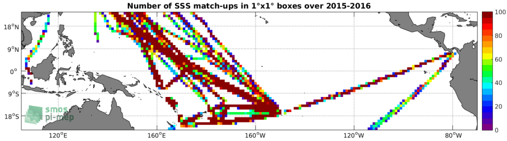
Figure 4: Number of SSS match-ups between TSG-LEGOS-DM SSS and the SMAP-L3-RSS-V3-MONTHLY-70KM SSS product for the Tropical Pacific Ocean Pi-MEP region over 1^\circ \times 1^\circ boxes and for the full satellite product period.
