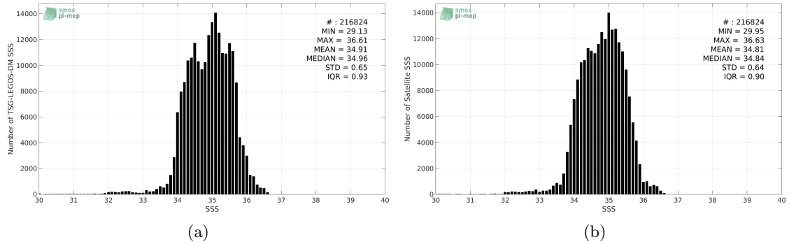
Figure 2: Histograms of SSS from TSG-LEGOS-DM (a) and SMAP-L3-RSS-V3-MONTHLY-70KM (b) considering all match-up pairs per bins of 0.1 over the Tropical Pacific Ocean Pi-MEP region and for the full satellite product period.
