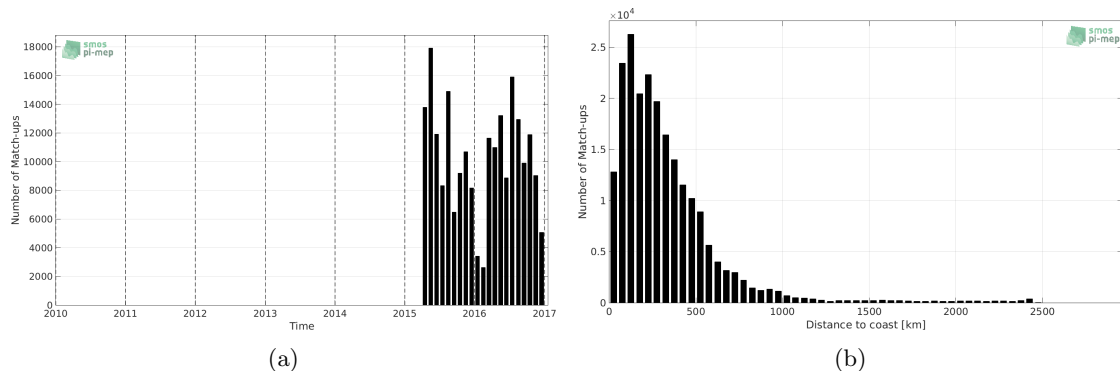
Figure 1: Number of match-ups between TSG-LEGOS-DM and SMAP-L3-RSS-V3-MONTHLY-70KM SSS as a function of time (a) and as function of the distance to coast (b) over the Tropical Pacific Ocean Pi-MEP region and for the full satellite product period.
