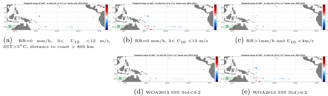
Figure 12: Temporal mean gridded over spatial boxes of size 1^\circ \times 1^\circ of \Delta SSS (SMAP-L3-RSS-V3-MONTHLY-70KM - TSG-GOSUD-Research-vessel) for 5 different subdatasets corresponding to: RR=0 mm/h, 3 < U_{10} < 12 m/s, SST > 5^\circ\text{C} , distance to coast > 800 km (a), RR=0 mm/h, 3 < U_{10} < 12 m/s (b), RR > 1 mm/h and U_{10} < 4 m/s (c), WOA2013 SSS Std < 0.2 (d), WOA2013 SSS Std > 0.2 (e).
