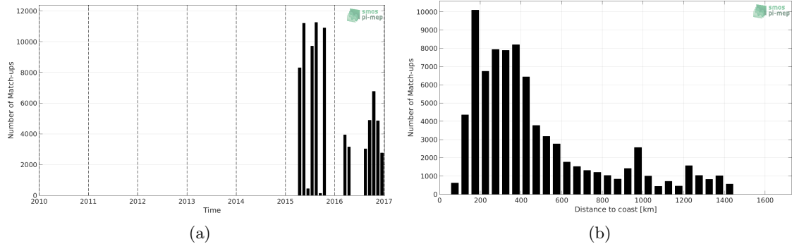
Figure 1: Number of match-ups between TSG-GOSUD-Research-vessel and SMAP-L3-RSS-V3-MONTHLY-70KM SSS as a function of time (a) and as function of the distance to coast (b) over the Tropical Pacific Ocean Pi-MEP region and for the full satellite product period.
