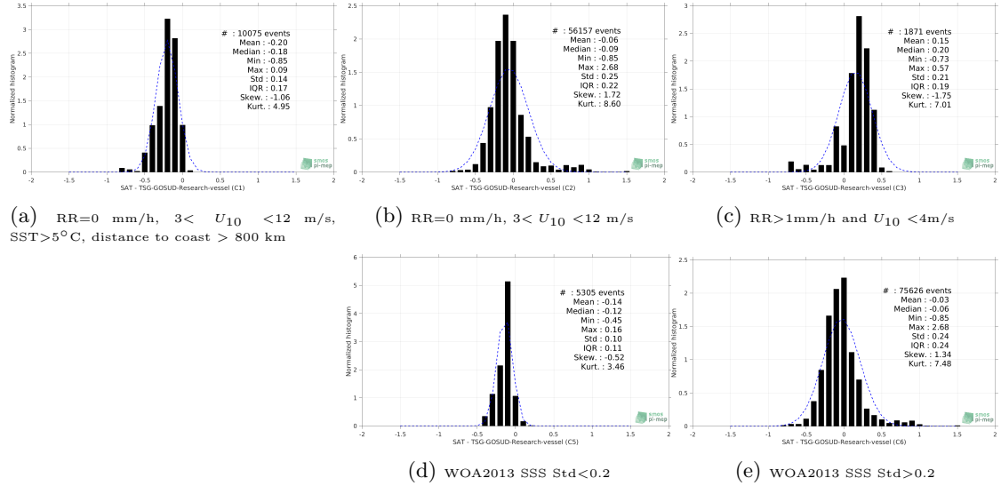
Figure 13: Normalized histogram of \Delta SSS (SMAP-L3-RSS-V3-MONTHLY-70KM - TSG-GOSUD-Research-vessel) for 5 different subdatasets corresponding to: RR=0 mm/h, 3 < U_{10} < 12 m/s, SST>5°C, distance to coast > 800 km (a), RR=0 mm/h, 3 < U_{10} < 12 m/s (b), RR>1mm/h and U_{10} < 4 m/s (c), WOA2013 SSS Std<0.2 (d), WOA2013 SSS Std>0.2 (e).
