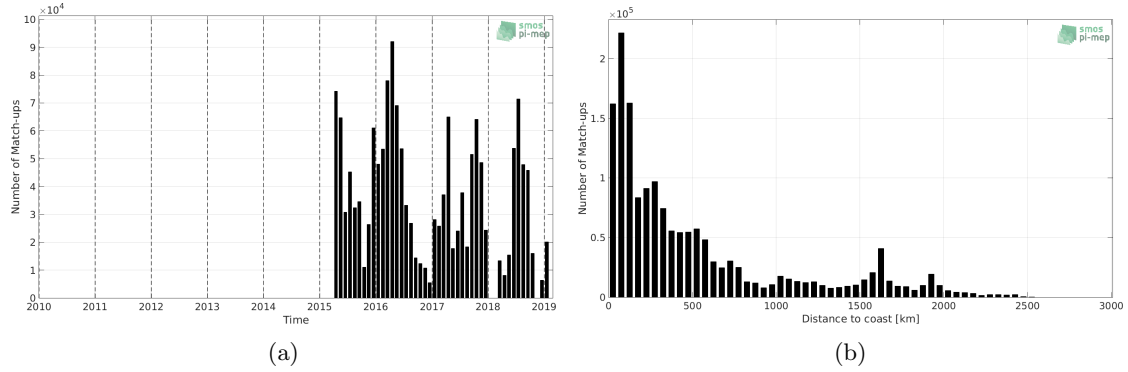
Figure 1: Number of match-ups between TSG-SAMOS and SMAP-L3-RSS-V3-MONTHLY-0.25DEG-40KM SSS as a function of time (a) and as function of the distance to coast (b) over the Tropical Pacific Ocean Pi-MEP region and for the full satellite product period.
