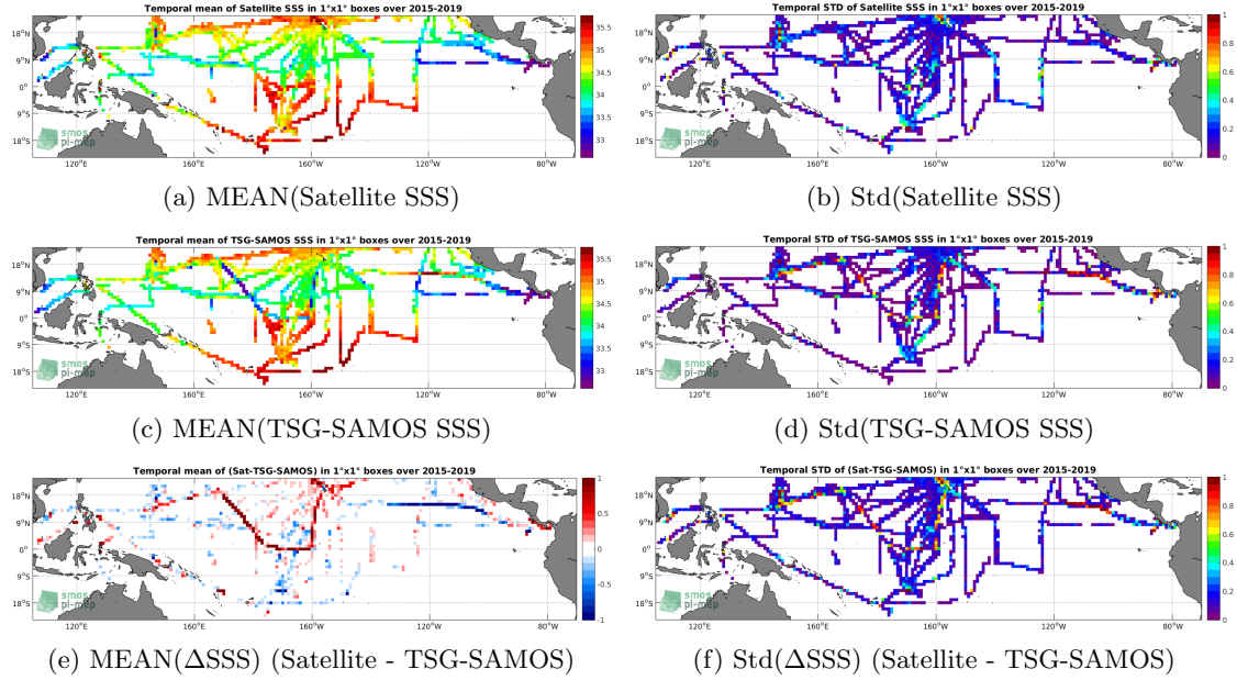
Figure 6: Temporal mean (left) and Std (right) of SSS from SMAP-L3-RSS-V3-MONTHLY-0.25DEG-40KM (top), TSG-SAMOS (middle), and of \Delta SSS (Satellite - TSG-SAMOS). Only match-up pairs are used to generate these maps.
