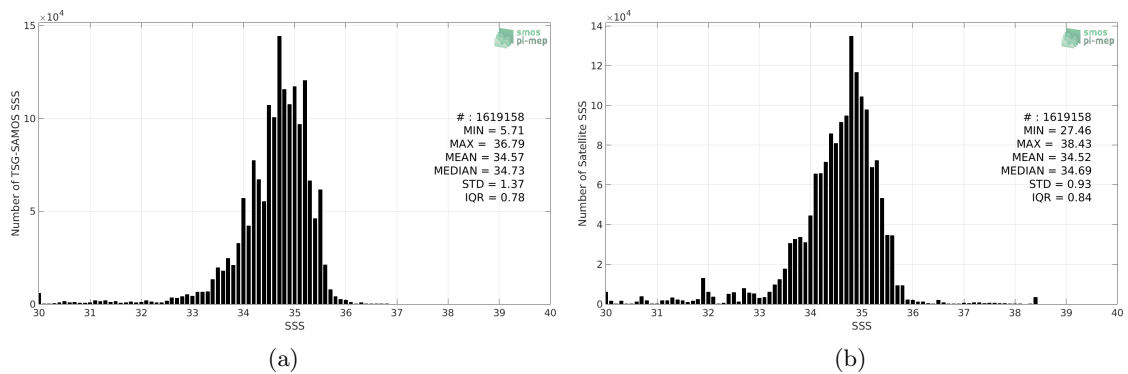
Figure 2: Histograms of SSS from TSG-SAMOS (a) and SMAP-L3-RSS-V3-MONTHLY-0.25DEG-40KM (b) considering all match-up pairs per bins of 0.1 over the Tropical Pacific Ocean Pi-MEP region and for the full satellite product period.
