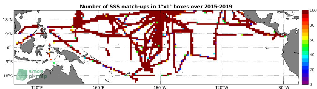
Figure 4: Number of SSS match-ups between TSG-SAMOS SSS and the SMAP-L3-RSS-V3-MONTHLY-0.25DEG-40KM SSS product for the Tropical Pacific Ocean Pi-MEP region over 1^\circ \times 1^\circ boxes and for the full satellite product period.
