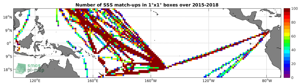
Figure 4: Number of SSS match-ups between TSG-LEGOS-DM SSS and the SMAP-L3-RSS-V3-MONTHLY-0.25DEG-40KM SSS product for the Tropical Pacific Ocean Pi-MEP region over 1^\circ \times 1^\circ boxes and for the full satellite product period.
