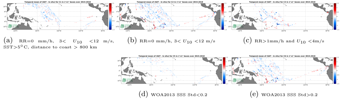
Figure 12: Temporal mean gridded over spatial boxes of size 1^\circ \times 1^\circ of \Delta SSS (SMAP-L3-RSS-V3-MONTHLY-0.25DEG-40KM - TSG-LEGOS-DM) for 5 different subdatasets corresponding to: RR=0 mm/h, 3 < U_{10} < 12 m/s, SST > 5^\circ C , distance to coast > 800 km (a), RR=0 mm/h, 3 < U_{10} < 12 m/s (b), RR > 1 mm/h and U_{10} < 4 m/s (c), WOA2013 SSS Std < 0.2 (d), WOA2013 SSS Std > 0.2 (e).
