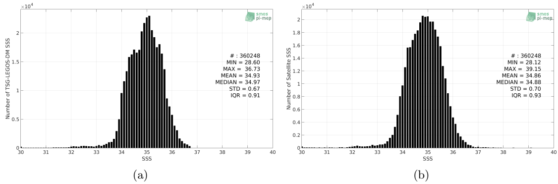
Figure 2: Histograms of SSS from TSG-LEGOS-DM (a) and SMAP-L3-RSS-V3-MONTHLY-0.25DEG-40KM (b) considering all match-up pairs per bins of 0.1 over the Tropical Pacific Ocean Pi-MEP region and for the full satellite product period.
