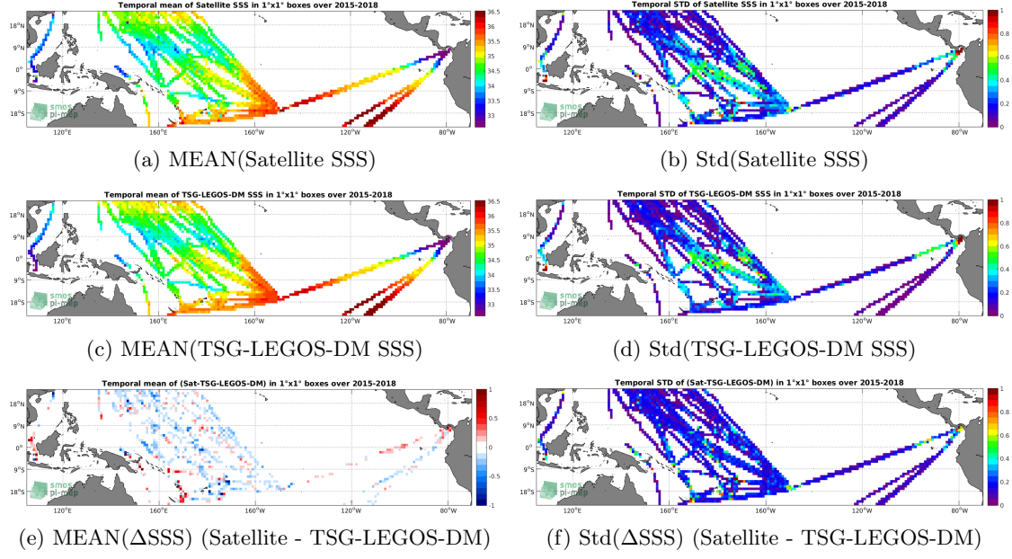
Figure 6: Temporal mean (left) and Std (right) of SSS from SMAP-L3-RSS-V3-MONTHLY-0.25DEG-40KM (top), TSG-LEGOS-DM (middle), and of \Delta SSS (Satellite - TSG-LEGOS-DM). Only match-up pairs are used to generate these maps.
