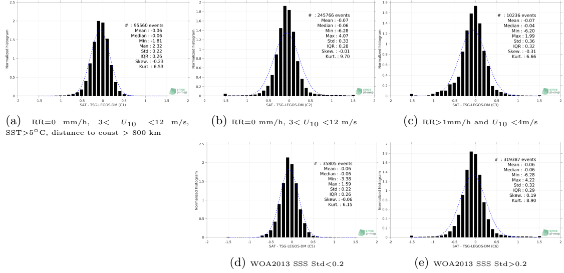
Figure 13: Normalized histogram of \Delta\text{SSS} (SMAP-L3-RSS-V3-MONTHLY-0.25DEG-40KM - TSG-LEGOS-DM) for 5 different subdatasets corresponding to: RR=0 mm/h, 3 < U_{10} < 12 m/s, SST >5^{\circ}\text{C} , distance to coast > 800 km (a), RR=0 mm/h, 3 < U_{10} < 12 m/s (b), RR>1\text{mm/h} and U_{10} < 4\text{m/s} (c), WOA2013 SSS Std <0.2 (d), WOA2013 SSS Std >0.2 (e).
