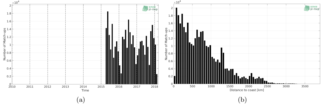
Figure 1: Number of match-ups between TSG-LEGOS-DM and SMAP-L3-RSS-V3-MONTHLY-0.25DEG-40KM SSS as a function of time (a) and as function of the distance to coast (b) over the Tropical Pacific Ocean Pi-MEP region and for the full satellite product period.
