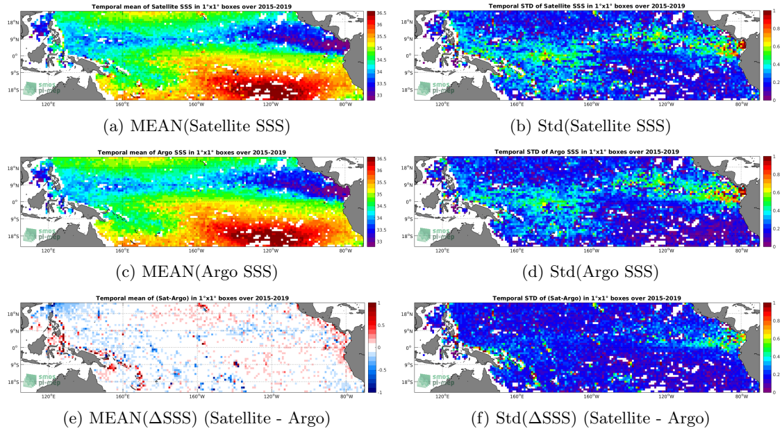
Figure 6: Temporal mean (left) and Std (right) of SSS from SMAP-L3-RSS-V3-MONTHLY-0.25DEG-40KM (top), Argo (middle), and of \Delta SSS (Satellite - Argo). Only match-up pairs are used to generate these maps.
