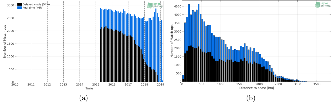
Figure 1: Number of match-ups between Argo and SMAP-L3-RSS-V3-MONTHLY-0.25DEG-40KM SSS as a function of time (a) and as function of the distance to coast (b) over the Tropical Pacific Ocean Pi-MEP region and for the full satellite product period.
