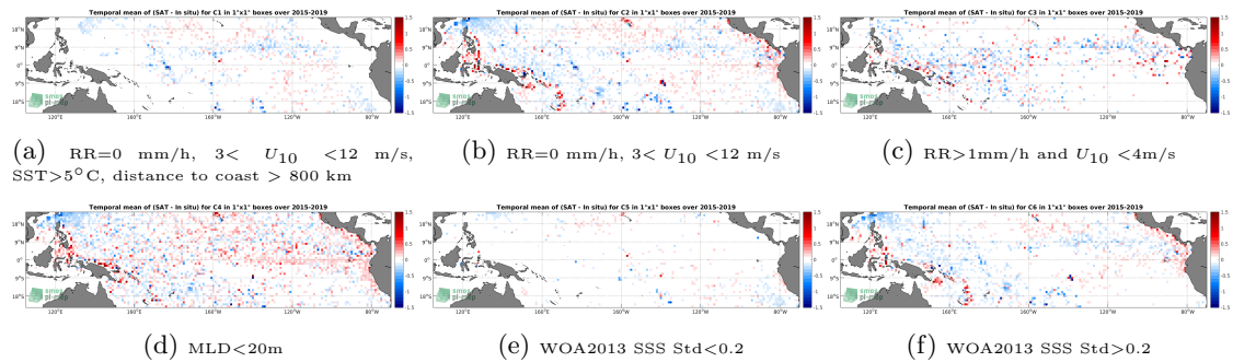
Figure 12: Temporal mean gridded over spatial boxes of size 1^\circ \times 1^\circ of \Delta SSS (SMAP-L3-RSS-V3-MONTHLY-0.25DEG-40KM - Argo) for 6 different subdatasets corresponding to:RR=0 mm/h, 3 < U_{10} < 12 m/s, SST > 5^\circ C, distance to coast > 800 km (a), RR=0 mm/h, 3 < U_{10} < 12 m/s (b), RR > 1 mm/h and U_{10} < 4 m/s (c),MLD < 20 m (d),WOA2013 SSS Std < 0.2 (e),WOA2013 SSS Std > 0.2 (f).
