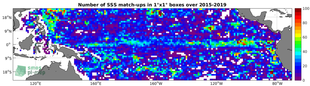
Figure 4: Number of SSS match-ups between Argo SSS and the SMAP-L3-RSS-V3-MONTHLY-0.25DEG-40KM SSS product for the Tropical Pacific Ocean Pi-MEP region over 1^\circ \times 1^\circ boxes and for the full satellite product period.
