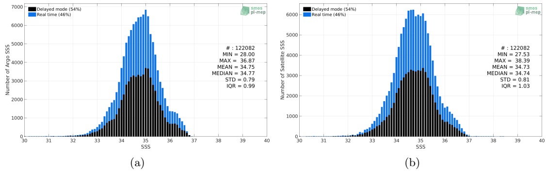
Figure 2: Histograms of SSS from Argo (a) and SMAP-L3-RSS-V3-MONTHLY-0.25DEG-40KM (b) considering all match-up pairs per bins of 0.1 over the Tropical Pacific Ocean Pi-MEP region and for the full satellite product period.
