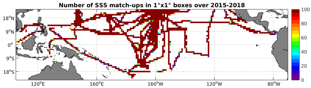
Figure 4: Number of SSS match-ups between TSG-SAMOS SSS and the SMAP-L3-RSS-V2-8DAY-RUNNING-40KM SSS product for the Tropical Pacific Ocean Pi-MEP region over 1^\circ \times 1^\circ boxes and for the full satellite product period.
