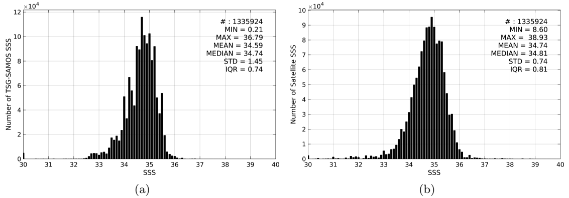
Figure 2: Histograms of SSS from TSG-SAMOS (a) and SMAP-L3-RSS-V2-8DAY-RUNNING-40KM (b) considering all match-up pairs per bins of 0.1 over the Tropical Pacific Ocean Pi-MEP region and for the full satellite product period.
