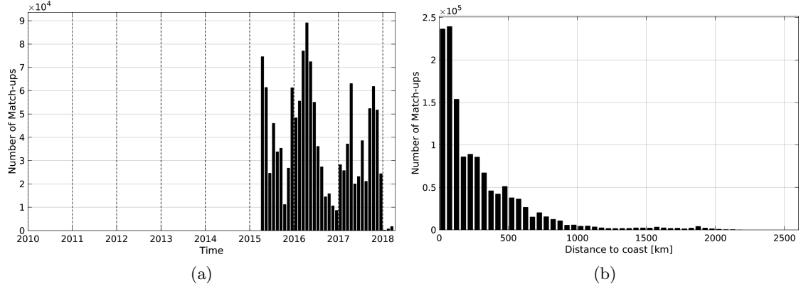
Figure 1: Number of match-ups between TSG-SAMOS and SMAP-L3-RSS-V2-8DAY-RUNNING-40KM SSS as a function of time (a) and as function of the distance to coast (b) over the Tropical Pacific Ocean Pi-MEP region and for the full satellite product period.
