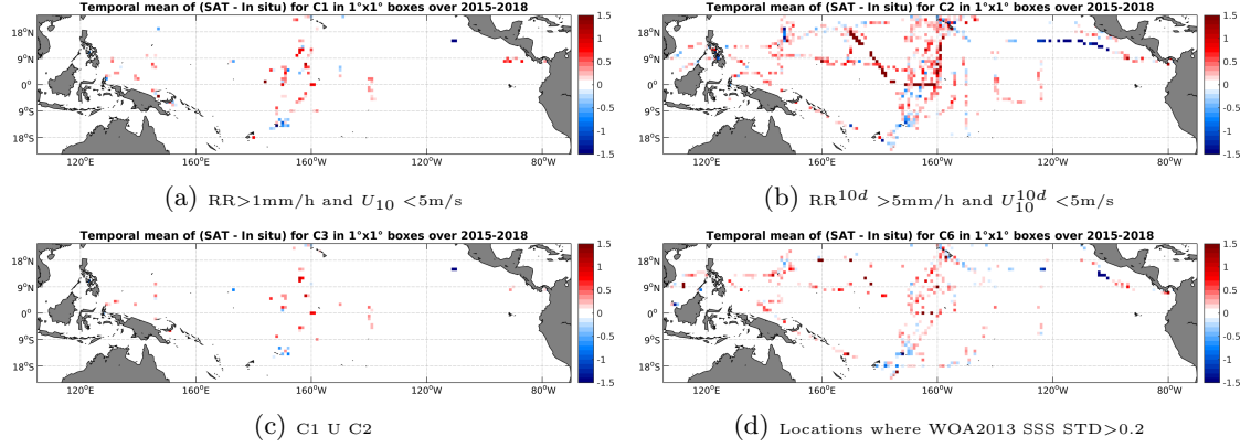
Figure 12: Temporal mean gridded over spatial boxes of size 1^\circ \times 1^\circ of \Delta SSS (SMAP-L3-RSS-V2-8DAY-RUNNING-40KM - TSG-SAMOS) for 4 different subdatasets corresponding to: RR > 1 mm/h and U_{10} < 5 m/s (a), RR^{10d} > 5 mm/h and U_{10}^{10d} < 5 m/s (b), C1 U C2 (c), Locations where WOA2013 SSS STD > 0.2 (d).
