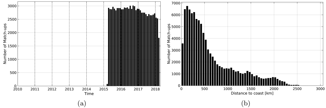
Figure 1: Number of match-ups between Argo and SMAP-L3-RSS-V2-8DAY-RUNNING-40KM SSS as a function of time (a) and as function of the distance to coast (b) over the Tropical Pacific Ocean Pi-MEP region and for the full satellite product period.
