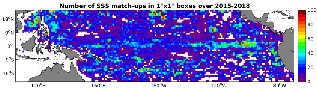
Figure 4: Number of SSS match-ups between Argo SSS and the SMAP-L3-RSS-V2-8DAY-RUNNING-40KM SSS product for the Tropical Pacific Ocean Pi-MEP region over 1^\circ \times 1^\circ boxes and for the full satellite product period.
