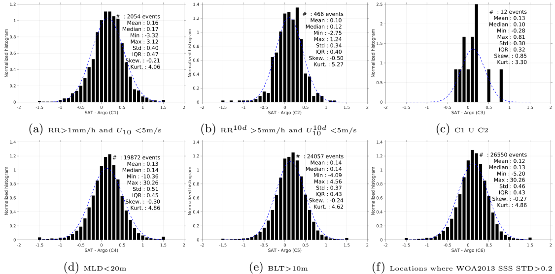
Figure 13: Normalized histogram of \Delta SSS (SMAP-L3-RSS-V2-8DAY-RUNNING-40KM - Argo) for 6 different subdatasets corresponding to: RR>1mm/h and U_{10} < 5m/s (a), RR^{10d} > 5mm/h and U_{10}^{10d} < 5m/s (b), C1 U C2 (c),MLD<20m (d),BLT>10m (e),Locations where WOA2013 SSS STD>0.2 (f).
