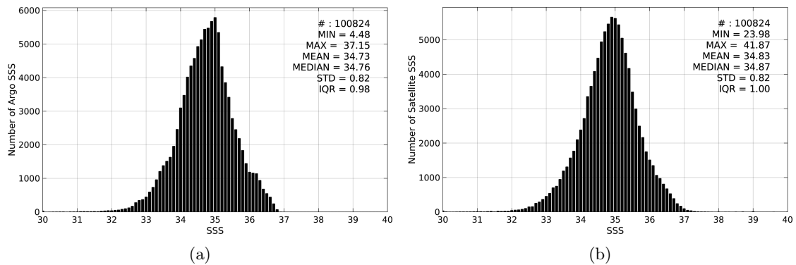
Figure 2: Histograms of SSS from Argo (a) and SMAP-L3-RSS-V2-8DAY-RUNNING-40KM (b) considering all match-up pairs per bins of 0.1 over the Tropical Pacific Ocean Pi-MEP region and for the full satellite product period.
