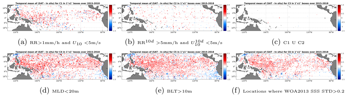
Figure 12: Temporal mean gridded over spatial boxes of size 1°x1° of \Delta SSS (SMAP-L3-RSS-V2-8DAY-RUNNING-40KM - Argo) for 6 different subdatasets corresponding to:RR>1mm/h and U_{10} < 5m/s (a), RR^{10d} > 5mm/h and U_{10}^{10d} < 5m/s (b), C1 U C2 (c),MLD<20m (d),BLT>10m (e),Locations where WOA2013 SSS STD>0.2 (f).
