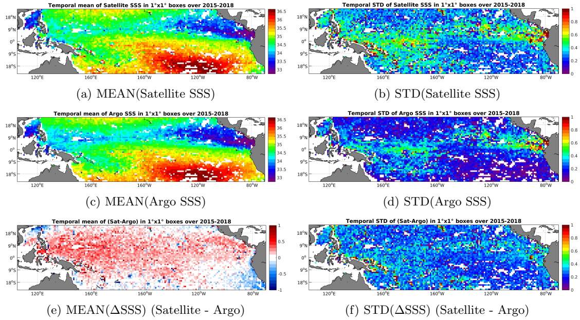
Figure 6: Temporal mean (left) and STD (right) of SSS from SMAP-L3-RSS-V2-8DAY-RUNNING-40KM (top), Argo (middle), and of \Delta SSS (Satellite - Argo). Only match-up pairs are used to generate these maps.
