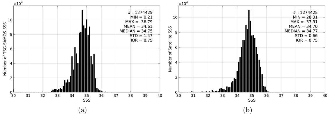
Figure 2: Histograms of SSS from TSG-SAMOS (a) and SMAP-L3-RSS-V2-8DAY-RUNNING-70KM (b) considering all match-up pairs per bins of 0.1 over the Tropical Pacific Ocean Pi-MEP region and for the full satellite product period.
