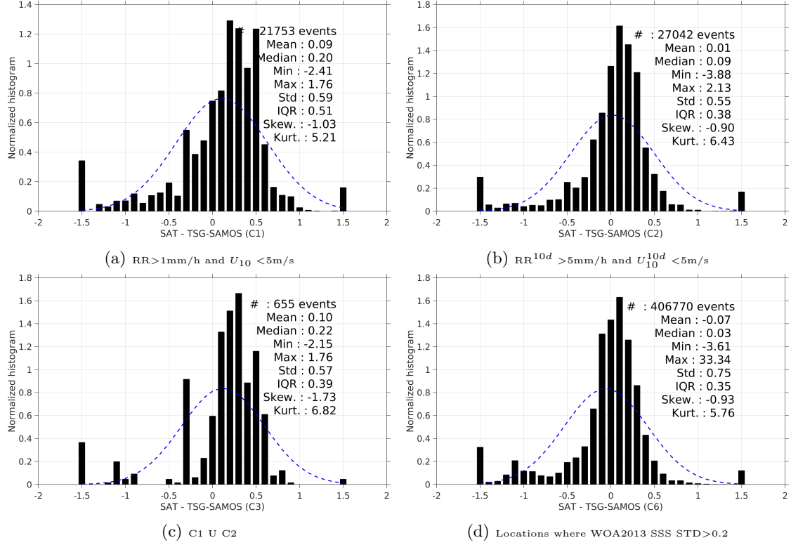
Figure 13: Normalized histogram of \Delta\text{SSS} (SMAP-L3-RSS-V2-8DAY-RUNNING-70KM - TSG-SAMOS) for 6 different subdatasets corresponding to: RR>1mm/h and U_{10} < 5\text{m/s} (a), RR^{10d} > 5\text{mm/h} and U_{10}^{10d} < 5\text{m/s} (b), C1 U C2 (c), Locations where WOA2013 SSS STD>0.2 (d).
