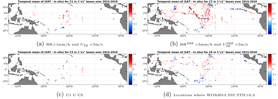
Figure 12: Temporal mean gridded over spatial boxes of size 1^\circ \times 1^\circ of \Delta SSS (SMAP-L3-RSS-V2-8DAY-RUNNING-70KM - TSG-SAMOS) for 4 different subdatasets corresponding to: RR > 1\text{mm/h} and U_{10} < 5\text{m/s} (a), RR^{10d} > 5\text{mm/h} and U_{10}^{10d} < 5\text{m/s} (b), C1 U C2 (c), Locations where WOA2013 SSS STD > 0.2 (d).
