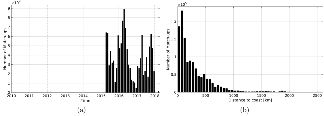
Figure 1: Number of match-ups between TSG-SAMOS and SMAP-L3-RSS-V2-8DAY-RUNNING-70KM SSS as a function of time (a) and as function of the distance to coast (b) over the Tropical Pacific Ocean Pi-MEP region and for the full satellite product period.
