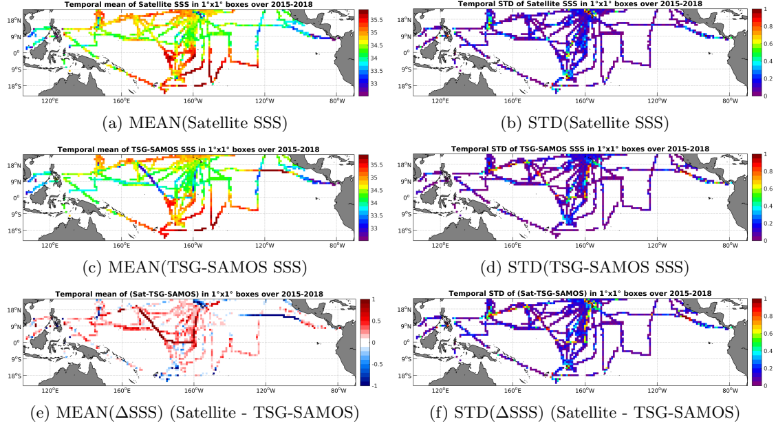
Figure 6: Temporal mean (left) and STD (right) of SSS from SMAP-L3-RSS-V2-8DAY-RUNNING-70KM (top), TSG-SAMOS (middle), and of \Delta SSS (Satellite - TSG-SAMOS). Only match-up pairs are used to generate these maps.
