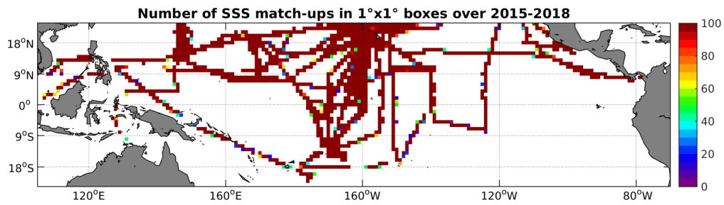
Figure 4: Number of SSS match-ups between TSG-SAMOS SSS and the SMAP-L3-RSS-V2-8DAY-RUNNING-70KM SSS product for the Tropical Pacific Ocean Pi-MEP region over 1^\circ \times 1^\circ boxes and for the full satellite product period.
