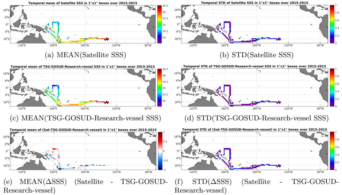
Figure 6: Temporal mean (left) and STD (right) of SSS from SMAP-L3-RSS-V2-8DAY-RUNNING-70KM (top), TSG-GOSUD-Research-vessel (middle), and of \Delta SSS (Satellite - TSG-GOSUD-Research-vessel). Only match-up pairs are used to generate these maps.
