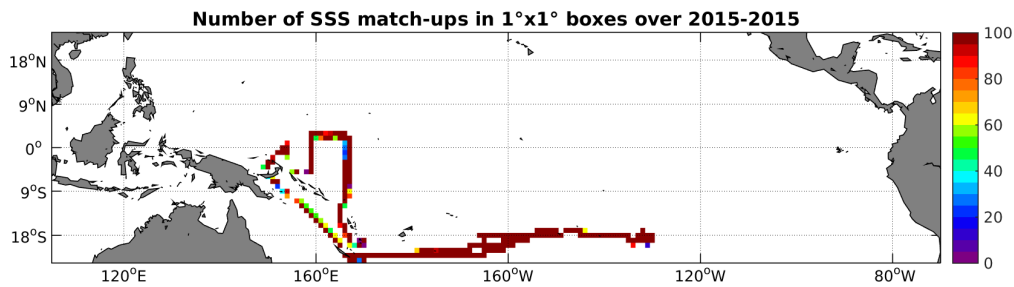
Figure 4: Number of SSS match-ups between TSG-GOSUD-Research-vessel SSS and the SMAP-L3-RSS-V2-8DAY-RUNNING-70KM SSS product for the Tropical Pacific Ocean Pi-MEP region over 1°x1° boxes and for the full satellite product period.
