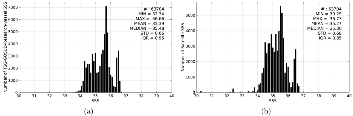
Figure 2: Histograms of SSS from TSG-GOSUD-Research-vessel (a) and SMAP-L3-RSS-V2-8DAY-RUNNING-70KM (b) considering all match-up pairs per bins of 0.1 over the Tropical Pacific Ocean Pi-MEP region and for the full satellite product period.
