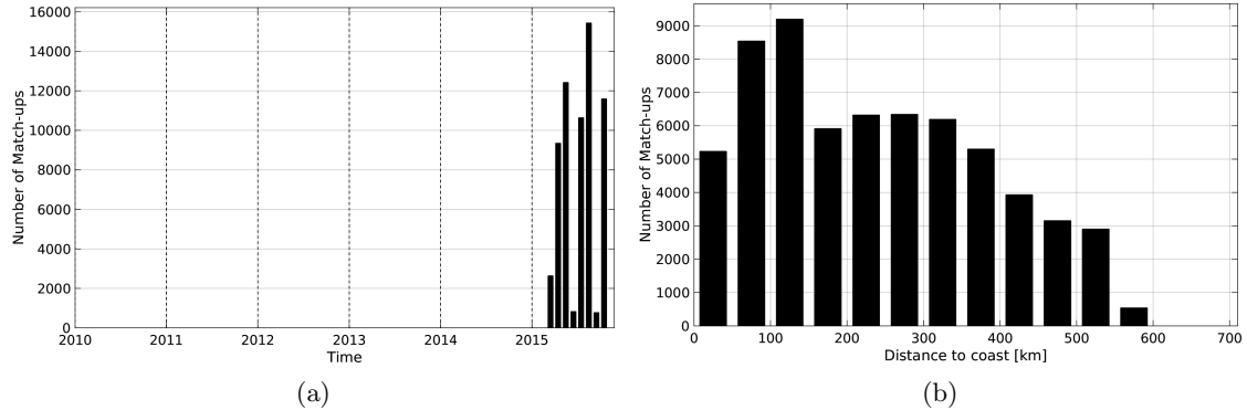
Figure 1: Number of match-ups between TSG-GOSUD-Research-vessel and SMAP-L3-RSS-V2-8DAY-RUNNING-70KM SSS as a function of time (a) and as function of the distance to coast (b) over the Tropical Pacific Ocean Pi-MEP region and for the full satellite product period.
