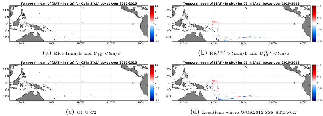
Figure 12: Temporal mean gridded over spatial boxes of size 1^\circ \times 1^\circ of \Delta SSS (SMAP-L3-RSS-V2-8DAY-RUNNING-70KM - TSG-GOSUD-Research-vessel) for 4 different subdatasets corresponding to: RR > 1 mm/h and U_{10} < 5 m/s (a), RR 10d > 5 mm/h and U_{10}^{10d} < 5 m/s (b), C1 U C2 (c), Locations where WOA2013 SSS STD > 0.2 (d).
