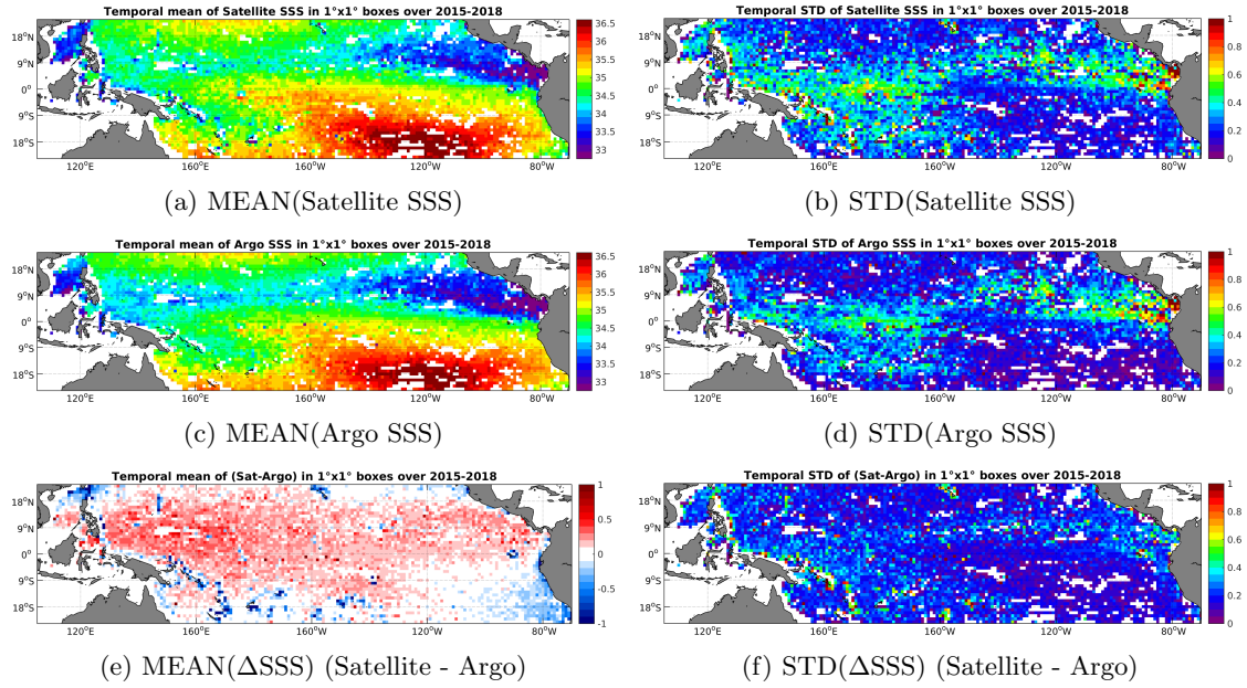
Figure 6: Temporal mean (left) and STD (right) of SSS from SMAP-L3-RSS-V2-8DAY-RUNNING-70KM (top), Argo (middle), and of \Delta SSS (Satellite - Argo). Only match-up pairs are used to generate these maps.
