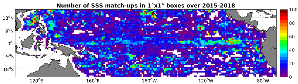
Figure 4: Number of SSS match-ups between Argo SSS and the SMAP-L3-RSS-V2-8DAY-RUNNING-70KM SSS product for the Tropical Pacific Ocean Pi-MEP region over 1^\circ \times 1^\circ boxes and for the full satellite product period.
