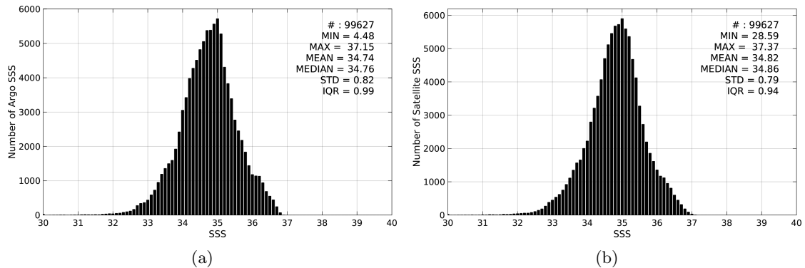
Figure 2: Histograms of SSS from Argo (a) and SMAP-L3-RSS-V2-8DAY-RUNNING-70KM (b) considering all match-up pairs per bins of 0.1 over the Tropical Pacific Ocean Pi-MEP region and for the full satellite product period.
