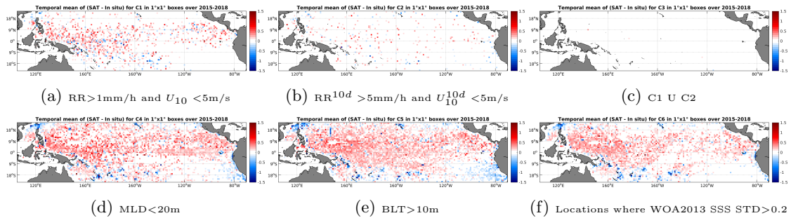
Figure 12: Temporal mean gridded over spatial boxes of size 1°x1° of \Delta SSS (SMAP-L3-RSS-V2-8DAY-RUNNING-70KM - Argo) for 6 different subdatasets corresponding to:RR>1mm/h and U_{10} < 5m/s (a), RR^{10d} > 5mm/h and U_{10}^{10d} < 5m/s (b), C1 U C2 (c),MLD<20m (d),BLT>10m (e),Locations where WOA2013 SSS STD>0.2 (f).
