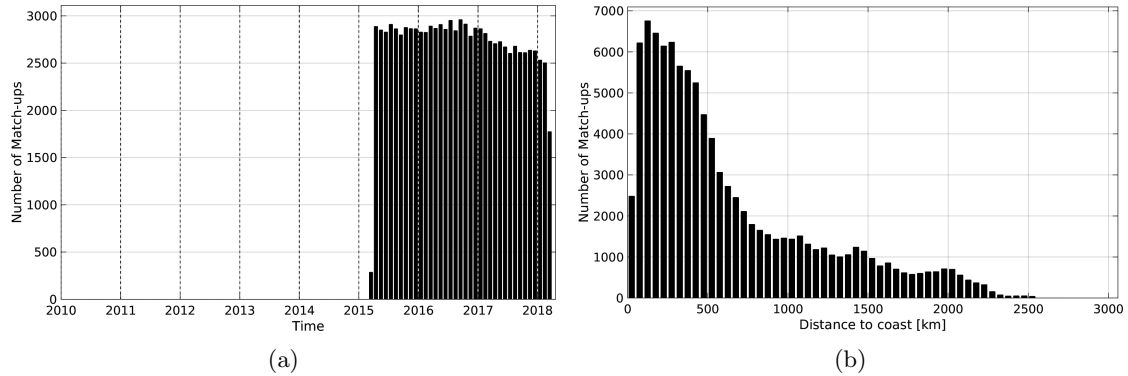
Figure 1: Number of match-ups between Argo and SMAP-L3-RSS-V2-8DAY-RUNNING-70KM SSS as a function of time (a) and as function of the distance to coast (b) over the Tropical Pacific Ocean Pi-MEP region and for the full satellite product period.
