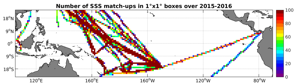
Figure 4: Number of SSS match-ups between TSG-LEGOS-DM SSS and the SMAP-L3-RSS-V2-MONTHLY-0.25DEG-40KM SSS product for the Tropical Pacific Ocean Pi-MEP region over 1^\circ \times 1^\circ boxes and for the full satellite product period.
