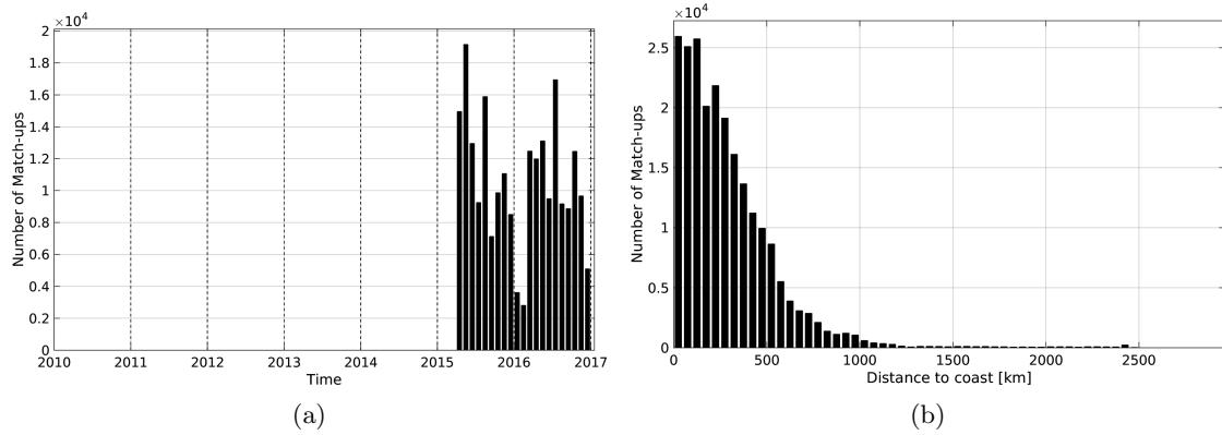
Figure 1: Number of match-ups between TSG-LEGOS-DM and SMAP-L3-RSS-V2-MONTHLY-0.25DEG-40KM SSS as a function of time (a) and as function of the distance to coast (b) over the Tropical Pacific Ocean Pi-MEP region and for the full satellite product period.
