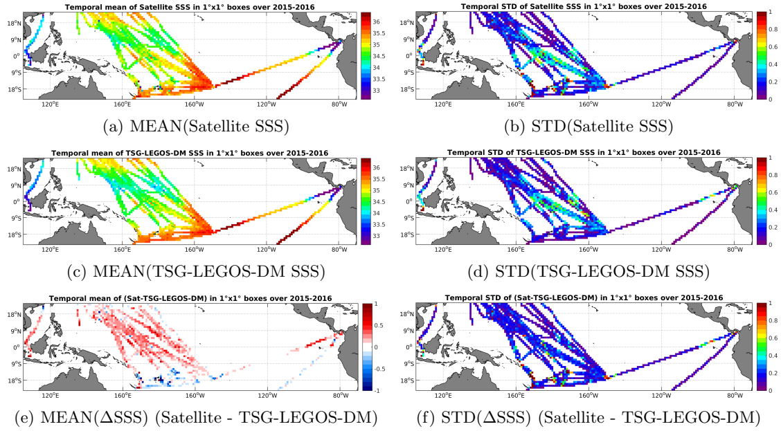
Figure 6: Temporal mean (left) and STD (right) of SSS from SMAP-L3-RSS-V2-MONTHLY-0.25DEG-40KM (top), TSG-LEGOS-DM (middle), and of \Delta SSS (Satellite - TSG-LEGOS-DM). Only match-up pairs are used to generate these maps.
