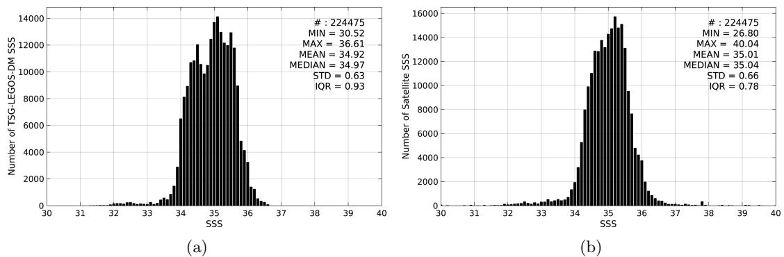
Figure 2: Histograms of SSS from TSG-LEGOS-DM (a) and SMAP-L3-RSS-V2-MONTHLY-0.25DEG-40KM (b) considering all match-up pairs per bins of 0.1 over the Tropical Pacific Ocean Pi-MEP region and for the full satellite product period.
