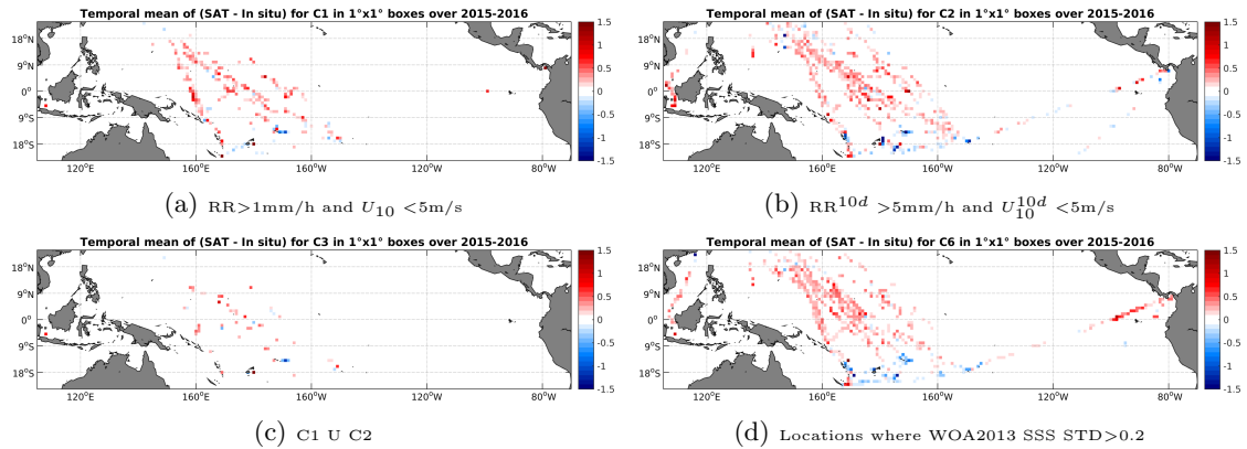
Figure 12: Temporal mean gridded over spatial boxes of size 1^\circ \times 1^\circ of \Delta SSS (SMAP-L3-RSS-V2-MONTHLY-0.25DEG-40KM - TSG-LEGOS-DM) for 4 different subdatasets corresponding to: RR > 1\text{mm/h} and U_{10} < 5\text{m/s} (a), RR^{10d} > 5\text{mm/h} and U_{10}^{10d} < 5\text{m/s} (b), C1 U C2 (c), Locations where WOA2013 SSS STD > 0.2 (d).
