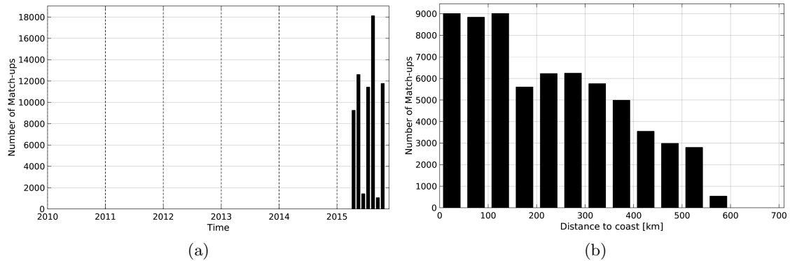
Figure 1: Number of match-ups between TSG-GOSUD-Research-vessel and SMAP-L3-RSS-V2-MONTHLY-0.25DEG-40KM SSS as a function of time (a) and as function of the distance to coast (b) over the Tropical Pacific Ocean Pi-MEP region and for the full satellite product period.
