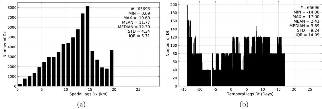
Figure 5: Histograms of the spatial (a) and temporal (b) lags between the time of the TSG-GOSUD-Research-vessel measurements and the date of the corresponding SMAP-L3-RSS-V2-MONTHLY-0.25DEG-40KM SSS product.
