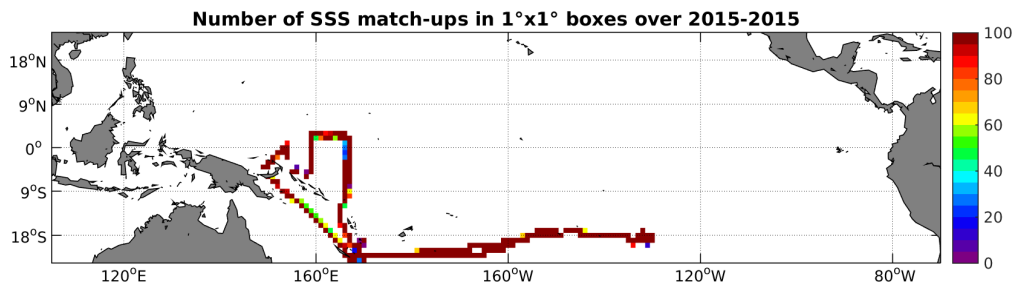
Figure 4: Number of SSS match-ups between TSG-GOSUD-Research-vessel SSS and the SMAP-L3-RSS-V2-MONTHLY-0.25DEG-40KM SSS product for the Tropical Pacific Ocean Pi-MEP region over 1^\circ \times 1^\circ boxes and for the full satellite product period.
