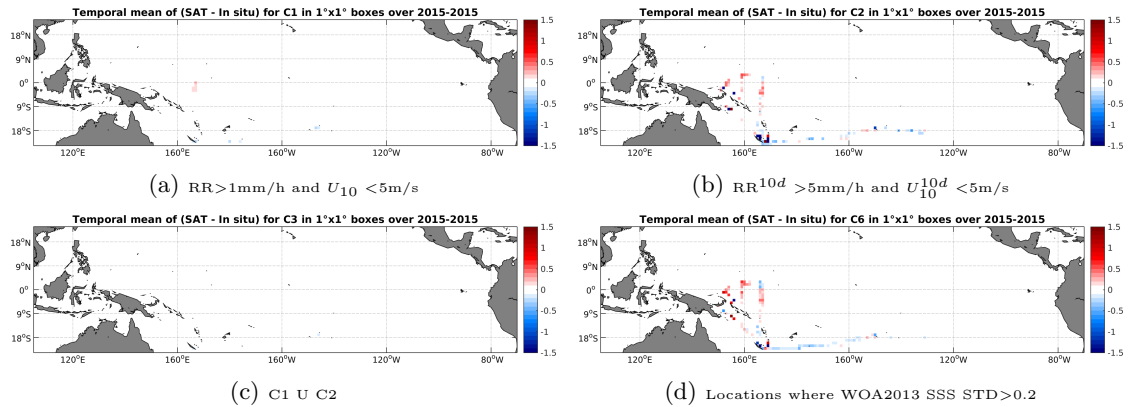
Figure 12: Temporal mean gridded over spatial boxes of size 1^\circ \times 1^\circ of \Delta SSS (SMAP-L3-RSS-V2-MONTHLY-0.25DEG-40KM - TSG-GOSUD-Research-vessel) for 4 different subdatasets corresponding to: RR > 1 mm/h and U_{10} < 5 m/s (a), RR 10d > 5 mm/h and U_{10}^{10d} < 5 m/s (b), C1 U C2 (c), Locations where WOA2013 SSS STD > 0.2 (d).
