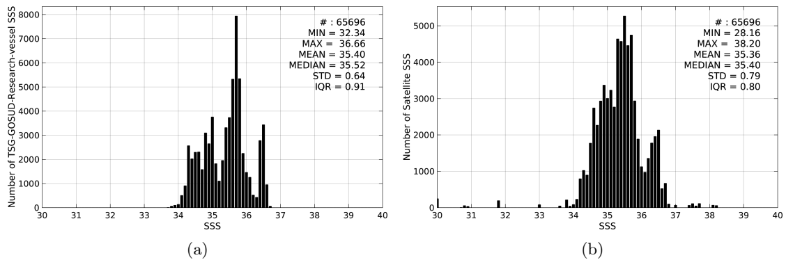
Figure 2: Histograms of SSS from TSG-GOSUD-Research-vessel (a) and SMAP-L3-RSS-V2-MONTHLY-0.25DEG-40KM (b) considering all match-up pairs per bins of 0.1 over the Tropical Pacific Ocean Pi-MEP region and for the full satellite product period.
