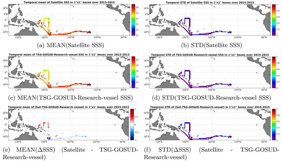
Figure 6: Temporal mean (left) and STD (right) of SSS from SMAP-L3-RSS-V2-MONTHLY-0.25DEG-40KM (top), TSG-GOSUD-Research-vessel (middle), and of \Delta SSS (Satellite - TSG-GOSUD-Research-vessel). Only match-up pairs are used to generate these maps.
