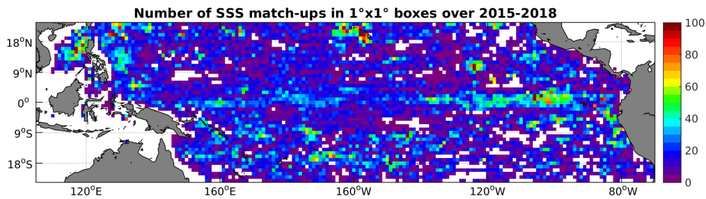
Figure 4: Number of SSS match-ups between Argo SSS and the SMAP-L3-RSS-V2-MONTHLY-0.25DEG-40KM SSS product for the Tropical Pacific Ocean Pi-MEP region over 1^\circ \times 1^\circ boxes and for the full satellite product period.
