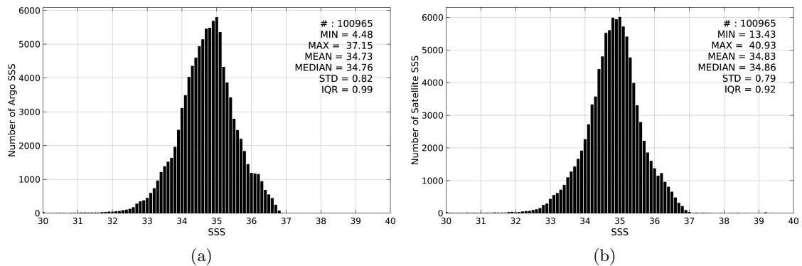
Figure 2: Histograms of SSS from Argo (a) and SMAP-L3-RSS-V2-MONTHLY-0.25DEG-40KM (b) considering all match-up pairs per bins of 0.1 over the Tropical Pacific Ocean Pi-MEP region and for the full satellite product period.
