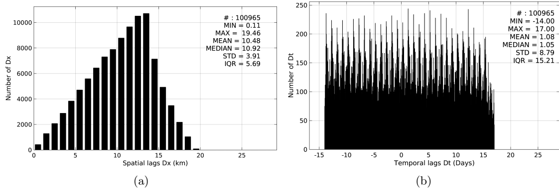
Figure 5: Histograms of the spatial (a) and temporal (b) lags between the time of the Argo measurements and the date of the corresponding SMAP-L3-RSS-V2-MONTHLY-0.25DEG-40KM SSS product.
