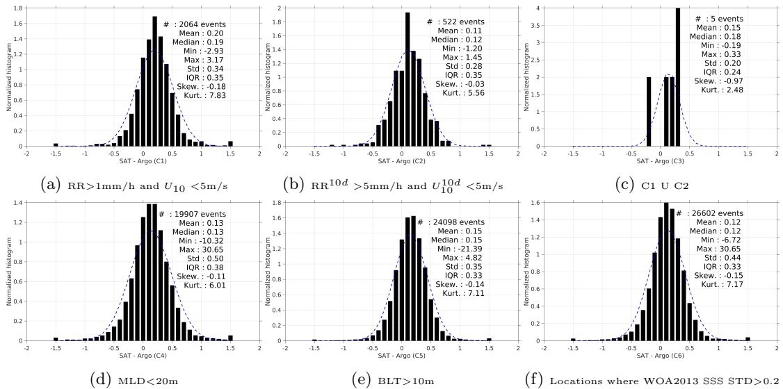
Figure 13: Normalized histogram of ΔSSS (SMAP-L3-RSS-V2-MONTHLY-0.25DEG-40KM - Argo) for 6 different subdatasets corresponding to: RR>1mm/h and U_{10} < 5\text{m/s} (a), RR^{10d} > 5\text{mm/h} and U_{10}^{10d} < 5\text{m/s} (b), C1 U C2 (c),MLD<20m (d),BLT>10m (e),Locations where WOA2013 SSS STD>0.2 (f).
