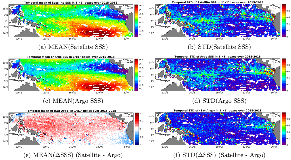
Figure 6: Temporal mean (left) and STD (right) of SSS from SMAP-L3-RSS-V2-MONTHLY-0.25DEG-40KM (top), Argo (middle), and of \Delta SSS (Satellite - Argo). Only match-up pairs are used to generate these maps.
