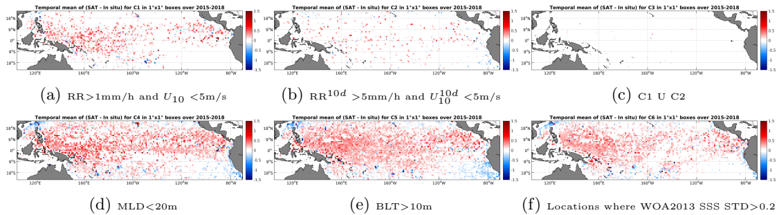
Figure 12: Temporal mean gridded over spatial boxes of size 1°x1° of ΔSSS (SMAP-L3-RSS-V2-MONTHLY-0.25DEG-40KM - Argo) for 6 different subdatasets corresponding to:RR>1mm/h and U_{10} < 5\text{m/s} (a), RR^{10d} > 5\text{mm/h} and U_{10}^{10d} < 5\text{m/s} (b), C1 U C2 (c),MLD<20m (d),BLT>10m (e),Locations where WOA2013 SSS STD>0.2 (f).
