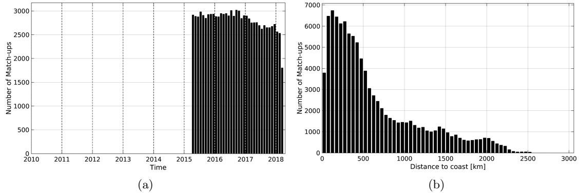
Figure 1: Number of match-ups between Argo and SMAP-L3-RSS-V2-MONTHLY-0.25DEG-40KM SSS as a function of time (a) and as function of the distance to coast (b) over the Tropical Pacific Ocean Pi-MEP region and for the full satellite product period.
