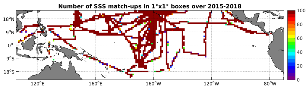
Figure 4: Number of SSS match-ups between TSG-SAMOS SSS and the SMAP-L3-RSS-V2-MONTHLY-70KM SSS product for the Tropical Pacific Ocean Pi-MEP region over 1^\circ \times 1^\circ boxes and for the full satellite product period.
