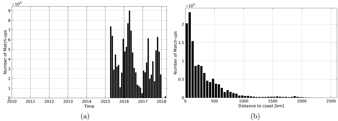
Figure 1: Number of match-ups between TSG-SAMOS and SMAP-L3-RSS-V2-MONTHLY-70KM SSS as a function of time (a) and as function of the distance to coast (b) over the Tropical Pacific Ocean Pi-MEP region and for the full satellite product period.
