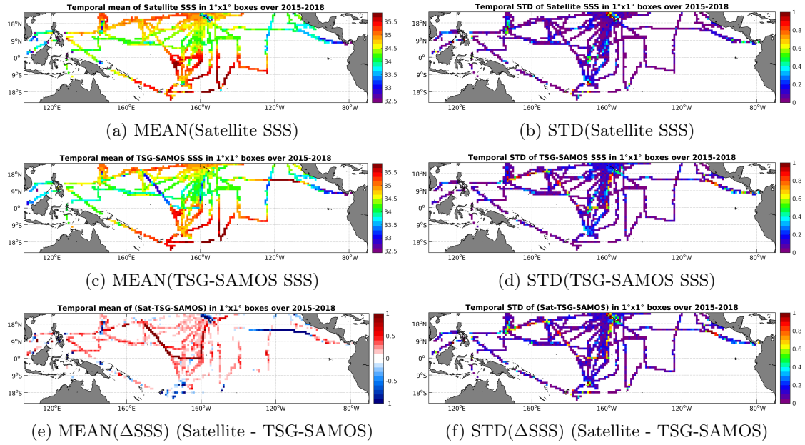
Figure 6: Temporal mean (left) and STD (right) of SSS from SMAP-L3-RSS-V2-MONTHLY-70KM (top), TSG-SAMOS (middle), and of \Delta SSS (Satellite - TSG-SAMOS). Only match-up pairs are used to generate these maps.
