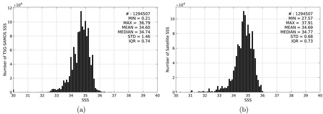
Figure 2: Histograms of SSS from TSG-SAMOS (a) and SMAP-L3-RSS-V2-MONTHLY-70KM (b) considering all match-up pairs per bins of 0.1 over the Tropical Pacific Ocean Pi-MEP region and for the full satellite product period.
