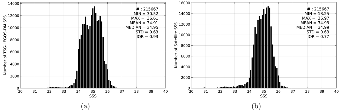
Figure 2: Histograms of SSS from TSG-LEGOS-DM (a) and SMAP-L3-RSS-V2-MONTHLY-70KM (b) considering all match-up pairs per bins of 0.1 over the Tropical Pacific Ocean Pi-MEP region and for the full satellite product period.
