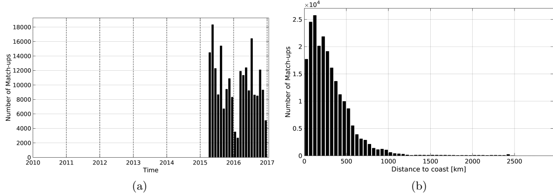
Figure 1: Number of match-ups between TSG-LEGOS-DM and SMAP-L3-RSS-V2-MONTHLY-70KM SSS as a function of time (a) and as function of the distance to coast (b) over the Tropical Pacific Ocean Pi-MEP region and for the full satellite product period.
