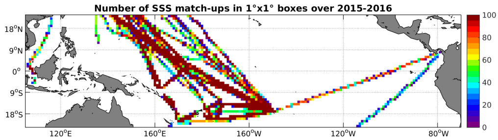
Figure 4: Number of SSS match-ups between TSG-LEGOS-DM SSS and the SMAP-L3-RSS-V2-MONTHLY-70KM SSS product for the Tropical Pacific Ocean Pi-MEP region over 1^\circ \times 1^\circ boxes and for the full satellite product period.
