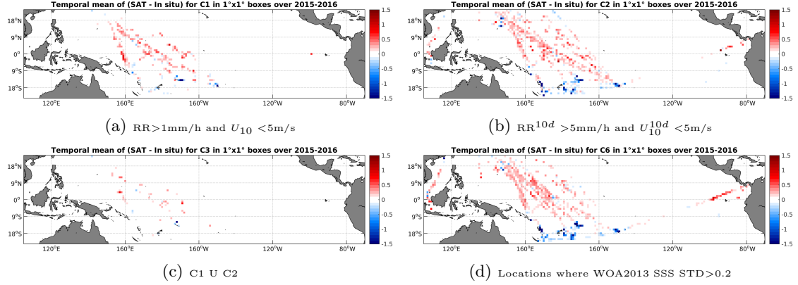
Figure 12: Temporal mean gridded over spatial boxes of size 1^\circ \times 1^\circ of \Delta SSS (SMAP-L3-RSS-V2-MONTHLY-70KM - TSG-LEGOS-DM) for 4 different subdatasets corresponding to: RR > 1\text{mm/h} and U_{10} < 5\text{m/s} (a), RR^{10d} > 5\text{mm/h} and U_{10}^{10d} < 5\text{m/s} (b), C1 U C2 (c), Locations where WOA2013 SSS STD > 0.2 (d).
