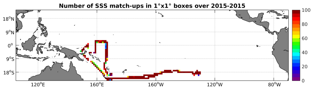
Figure 4: Number of SSS match-ups between TSG-GOSUD-Research-vessel SSS and the SMAP-L3-RSS-V2-MONTHLY-70KM SSS product for the Tropical Pacific Ocean Pi-MEP region over 1^\circ \times 1^\circ boxes and for the full satellite product period.
