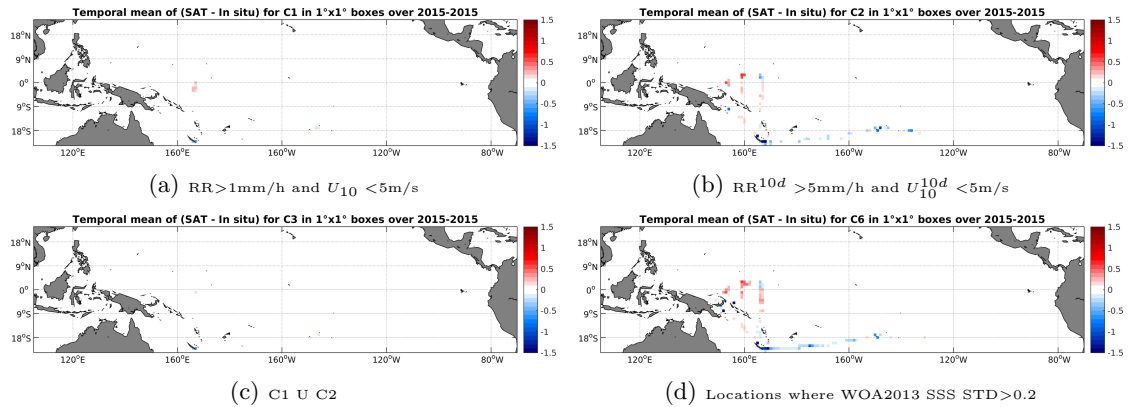
Figure 12: Temporal mean gridded over spatial boxes of size 1^\circ \times 1^\circ of \Delta SSS (SMAP-L3-RSS-V2-MONTHLY-70KM - TSG-GOSUD-Research-vessel) for 4 different subdatasets corresponding to:RR > 1 mm/h and U_{10} < 5 m/s (a), RR 10d > 5 mm/h and U_{10}^{10d} < 5 m/s (b), C1 U C2 (c),Locations where WOA2013 SSS STD > 0.2 (d).
