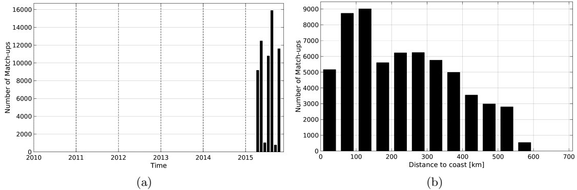
Figure 1: Number of match-ups between TSG-GOSUD-Research-vessel and SMAP-L3-RSS-V2-MONTHLY-70KM SSS as a function of time (a) and as function of the distance to coast (b) over the Tropical Pacific Ocean Pi-MEP region and for the full satellite product period.
