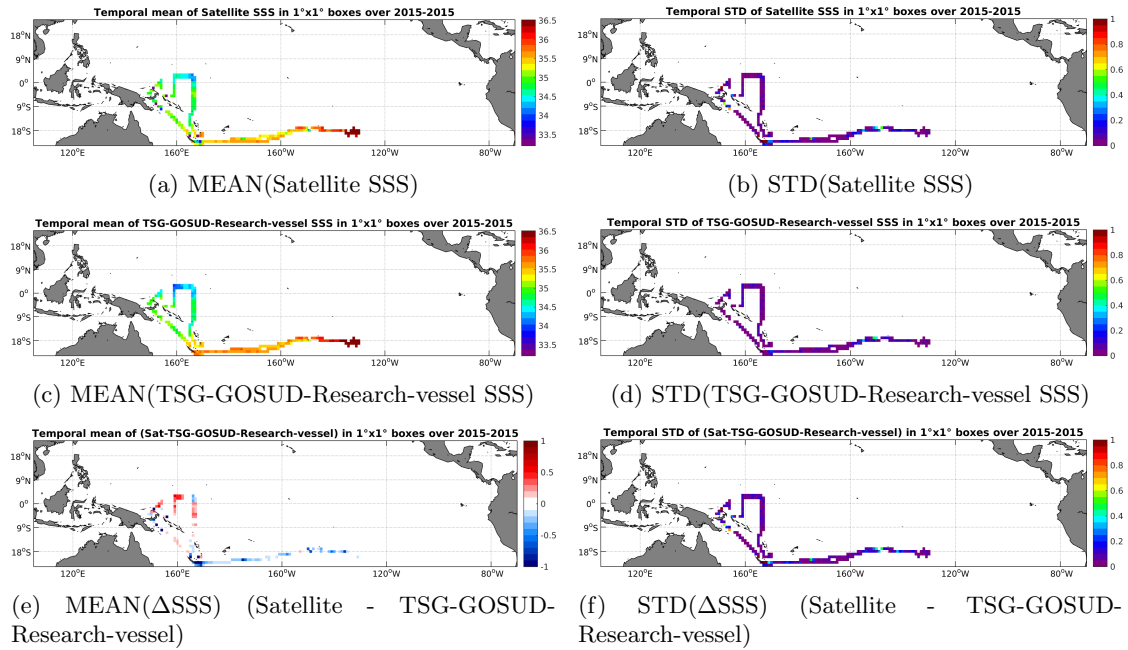
Figure 6: Temporal mean (left) and STD (right) of SSS from SMAP-L3-RSS-V2-MONTHLY-70KM (top), TSG-GOSUD-Research-vessel (middle), and of \Delta SSS (Satellite - TSG-GOSUD-Research-vessel). Only match-up pairs are used to generate these maps.
