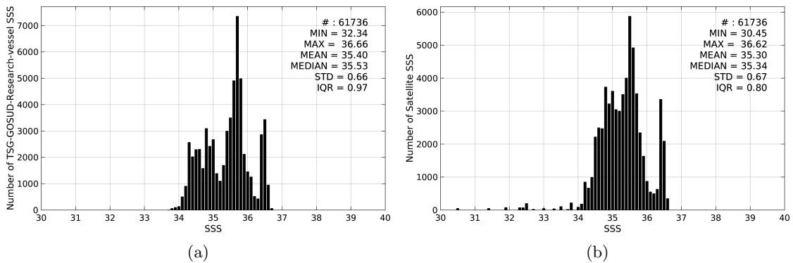
Figure 2: Histograms of SSS from TSG-GOSUD-Research-vessel (a) and SMAP-L3-RSS-V2-MONTHLY-70KM (b) considering all match-up pairs per bins of 0.1 over the Tropical Pacific Ocean Pi-MEP region and for the full satellite product period.
