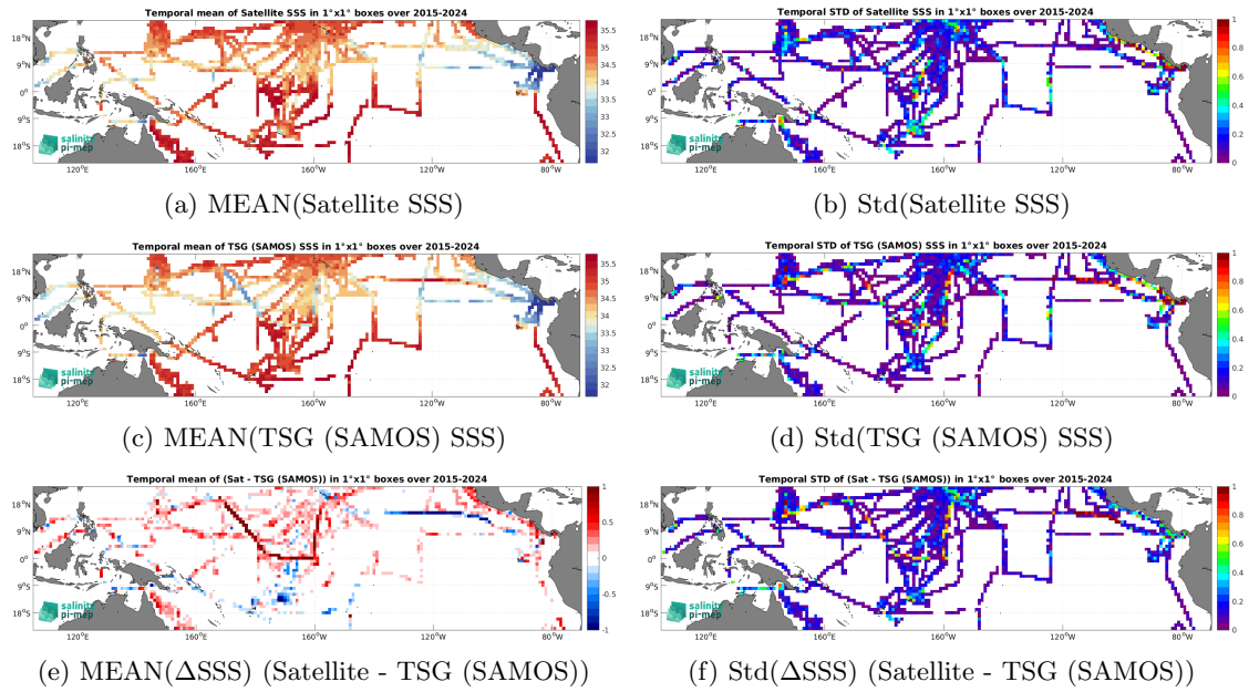
Figure 7: Temporal mean (left) and Std (right) of SSS from SMAP SSS L3 v5.0 - 8-Day running (JPL) (top), TSG (SAMOS) (middle), and of \Delta SSS (Satellite - TSG (SAMOS)). Only match-up pairs are used to generate these maps.
