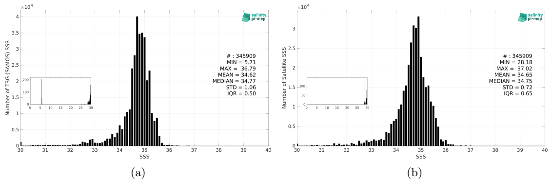
Figure 3: Histograms of SSS from TSG (SAMOS) (a) and SMAP SSS L3 v5.0 - 8-Day running (JPL) (b) considering all match-up pairs per bins of 0.1 over the Tropical Pacific Ocean Pi-MEP region and for the full satellite product period.
