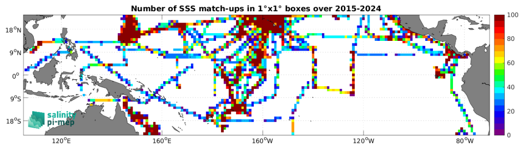
Figure 5: Number of SSS match-ups between TSG (SAMOS) SSS and the SMAP SSS L3 v5.0 - 8-Day running (JPL) SSS product for the Tropical Pacific Ocean Pi-MEP region over 1^\circ \times 1^\circ boxes and for the full satellite product period.
