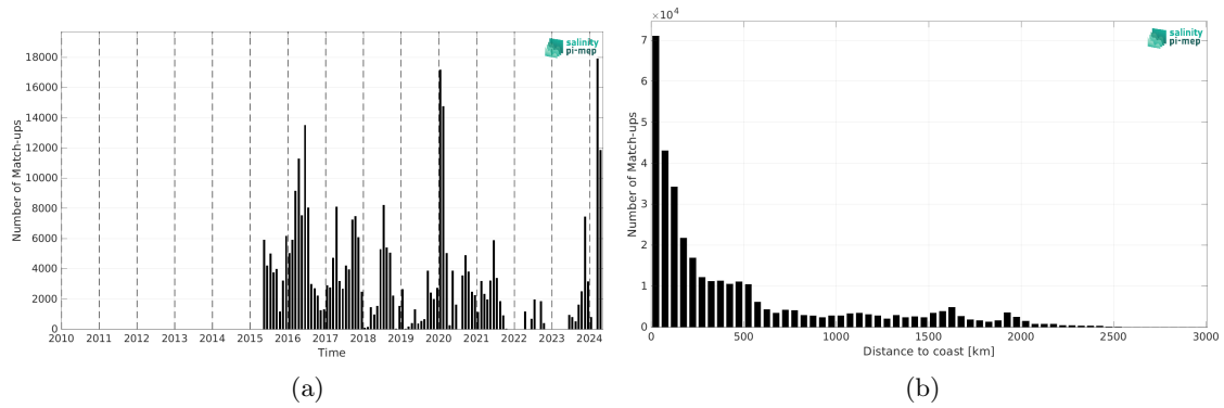
Figure 2: Number of match-ups between TSG (SAMOS) and SMAP SSS L3 v5.0 - 8-Day running (JPL) SSS as a function of time (a) and as function of the distance to coast (b) over the Tropical Pacific Ocean Pi-MEP region and for the full satellite product period.
