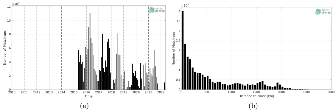
Figure 1: Number of match-ups between TSG (SAMOS) and SMAP SSS L3 v5.0 - 8-Day running (JPL) SSS as a function of time (a) and as function of the distance to coast (b) over the Tropical Pacific Ocean Pi-MEP region and for the full satellite product period.
