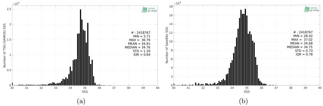
Figure 2: Histograms of SSS from TSG (SAMOS) (a) and SMAP SSS L3 v5.0 - 8-Day running (JPL) (b) considering all match-up pairs per bins of 0.1 over the Tropical Pacific Ocean Pi-MEP region and for the full satellite product period.
