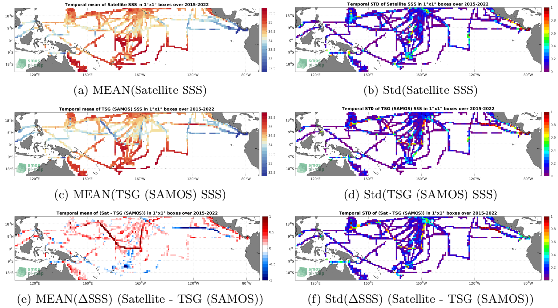
Figure 6: Temporal mean (left) and Std (right) of SSS from SMAP SSS L3 v5.0 - 8-Day running (JPL) (top), TSG (SAMOS) (middle), and of \Delta SSS (Satellite - TSG (SAMOS)). Only match-up pairs are used to generate these maps.
