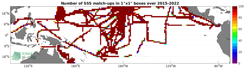
Figure 4: Number of SSS match-ups between TSG (SAMOS) SSS and the SMAP SSS L3 v5.0 - 8-Day running (JPL) SSS product for the Tropical Pacific Ocean Pi-MEP region over 1^\circ \times 1^\circ boxes and for the full satellite product period.
