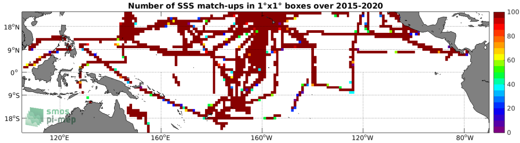
Figure 4: Number of SSS match-ups between TSG (SAMOS) SSS and the SMAP SSS L3 v5.0 - 8-Day running (JPL) SSS product for the Tropical Pacific Ocean Pi-MEP region over 1^\circ \times 1^\circ boxes and for the full satellite product period.
