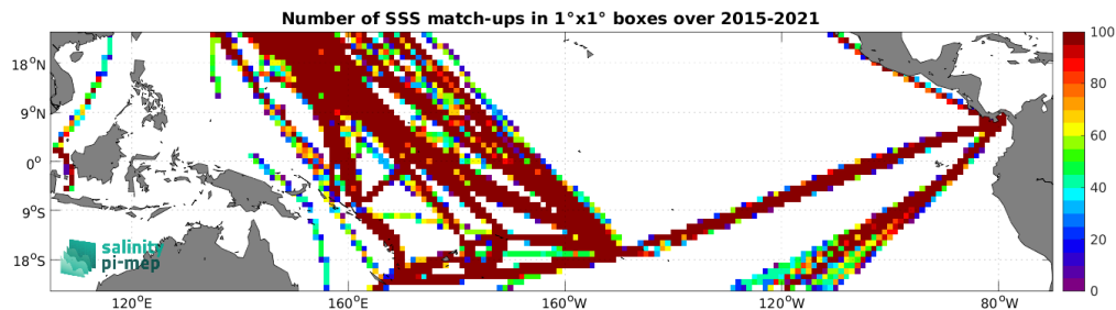
Figure 4: Number of SSS match-ups between TSG (LEGOS-DM) SSS and the SMAP SSS L3 v5.0 - 8-Day running (JPL) SSS product for the Tropical Pacific Ocean Pi-MEP region over 1^\circ \times 1^\circ boxes and for the full satellite product period.
