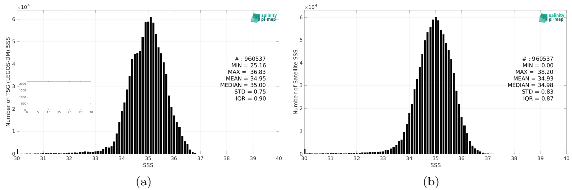
Figure 2: Histograms of SSS from TSG (LEGOS-DM) (a) and SMAP SSS L3 v5.0 - 8-Day running (JPL) (b) considering all match-up pairs per bins of 0.1 over the Tropical Pacific Ocean Pi-MEP region and for the full satellite product period.
