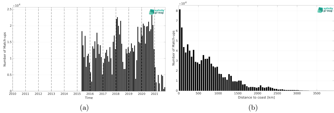
Figure 1: Number of match-ups between TSG (LEGOS-DM) and SMAP SSS L3 v5.0 - 8-Day running (JPL) SSS as a function of time (a) and as function of the distance to coast (b) over the Tropical Pacific Ocean Pi-MEP region and for the full satellite product period.
